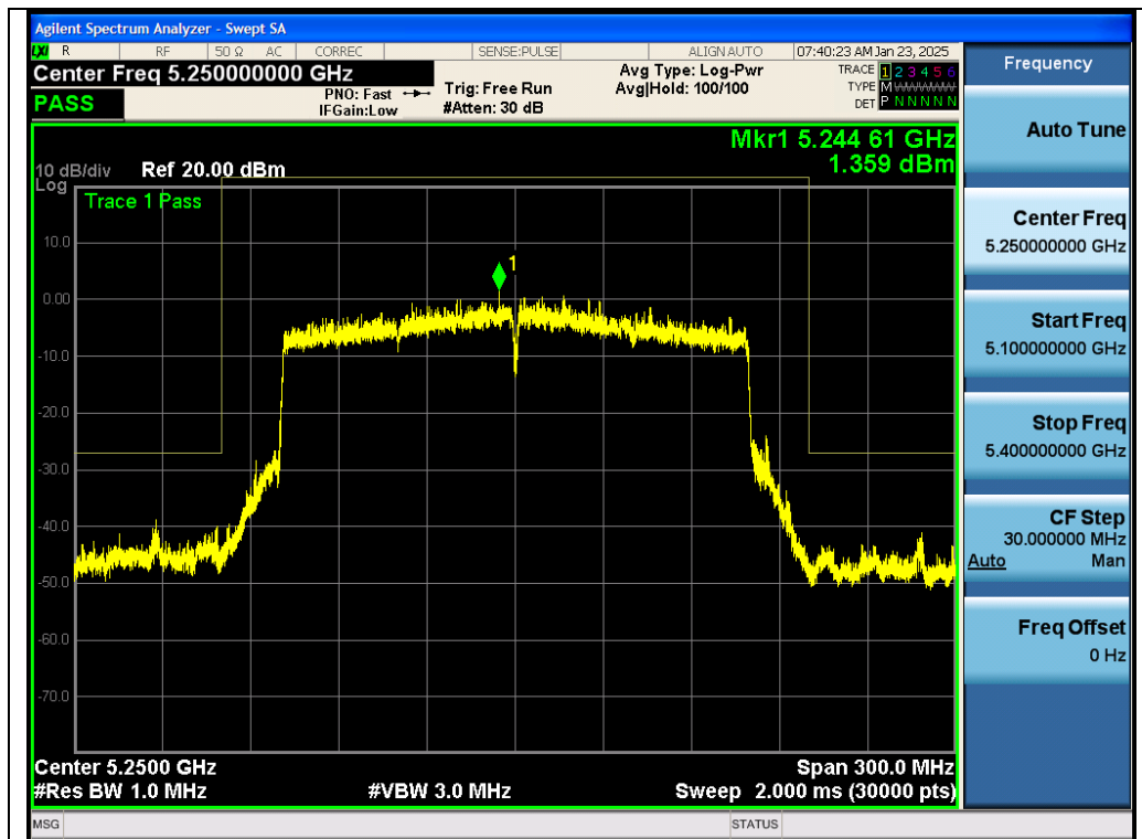
Test_Graph_802.11ax160_Chain A_5250_MCS0_Frequency Band 3
