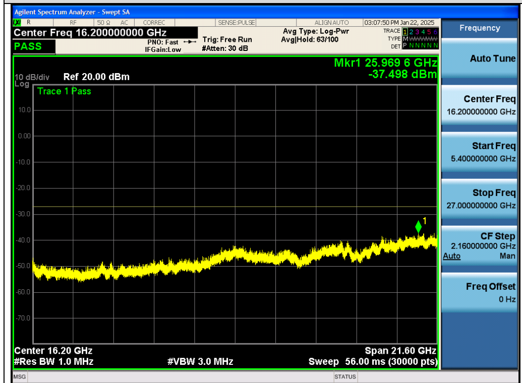
Test_Graph_802.11n40_Chain A_5270_MCS0_Frequency Band 4
