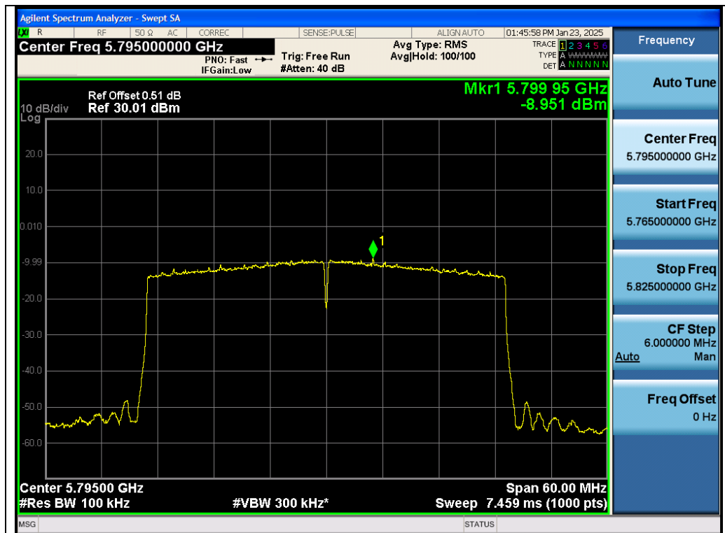
Test_Graph_802.11ax40_Chain B_5795_MCS0_PSD
