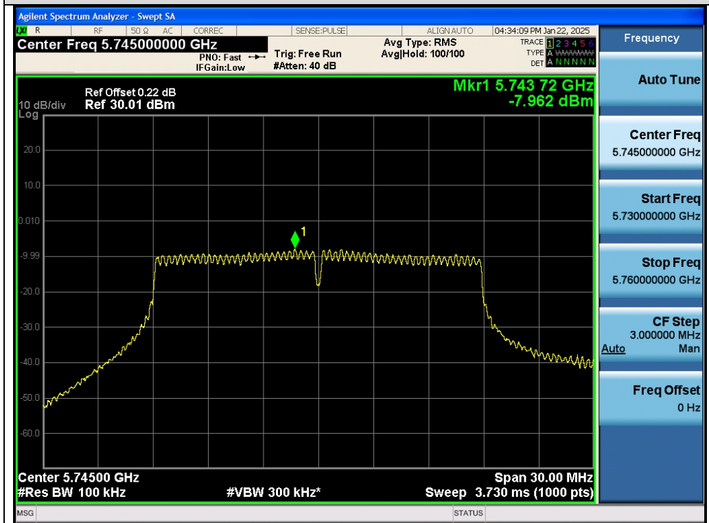
Test_Graph_802.11n20_Chain A_5745_MCS0_PSD
