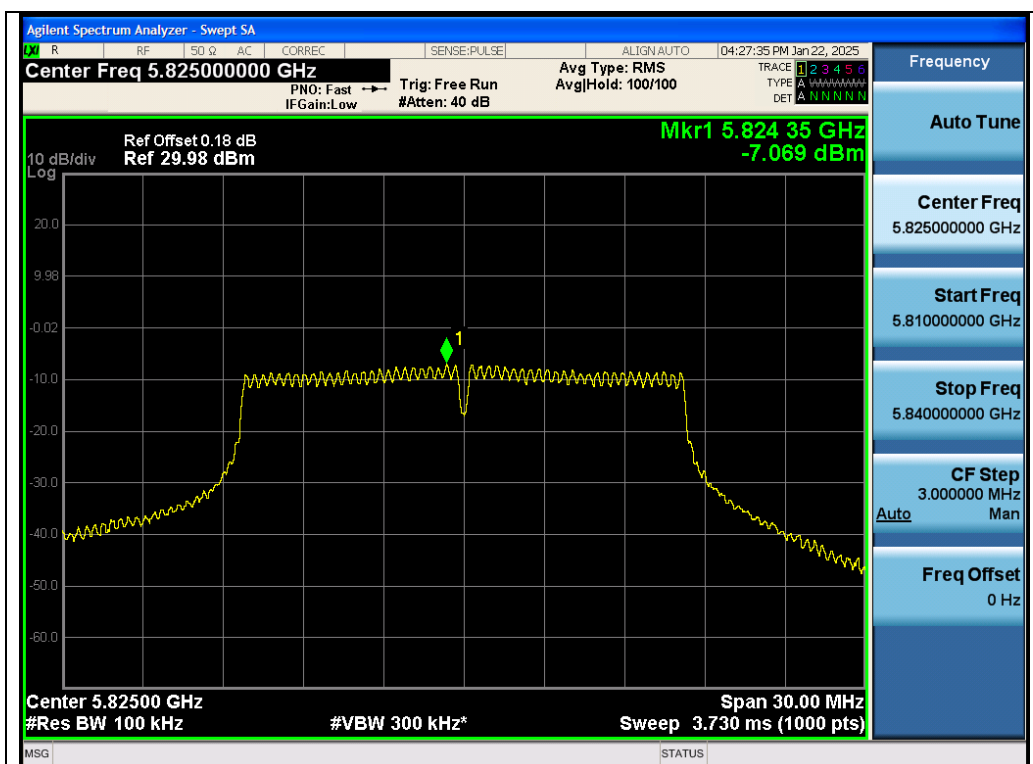
Test_Graph_802.11a_Chain A_5825_6Mbps_PSD
