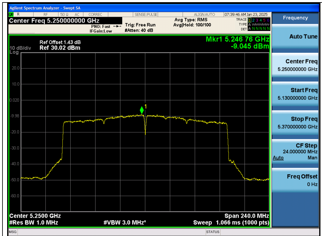
Test_Graph_802.11ax160_Chain A_5250_MCS0_PSD
