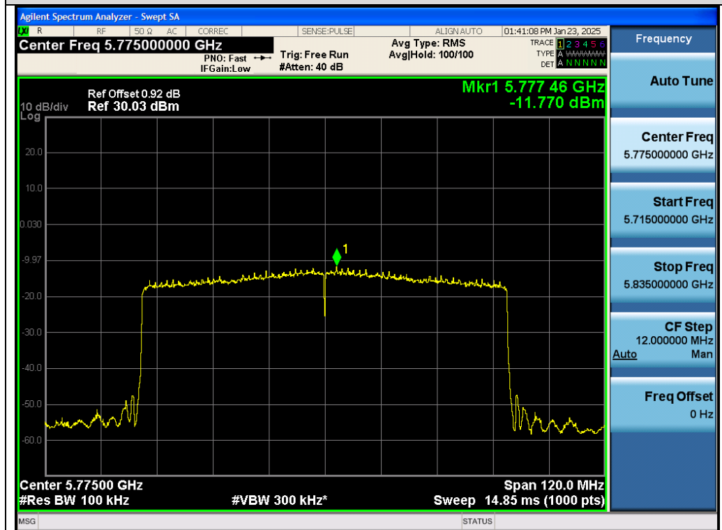
Test_Graph_802.11ax80_Chain B_5775_MCS0_PSD
