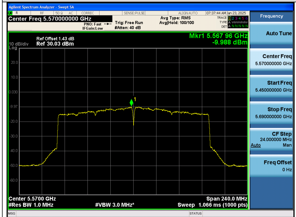
Test_Graph_802.11ax160_Chain A_5570_MCS0_PSD
