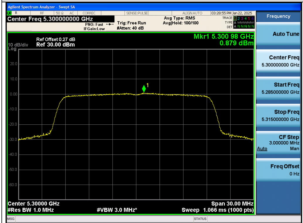
Test_Graph_802.11ax20_Chain A_5300_MCS0_PSD
