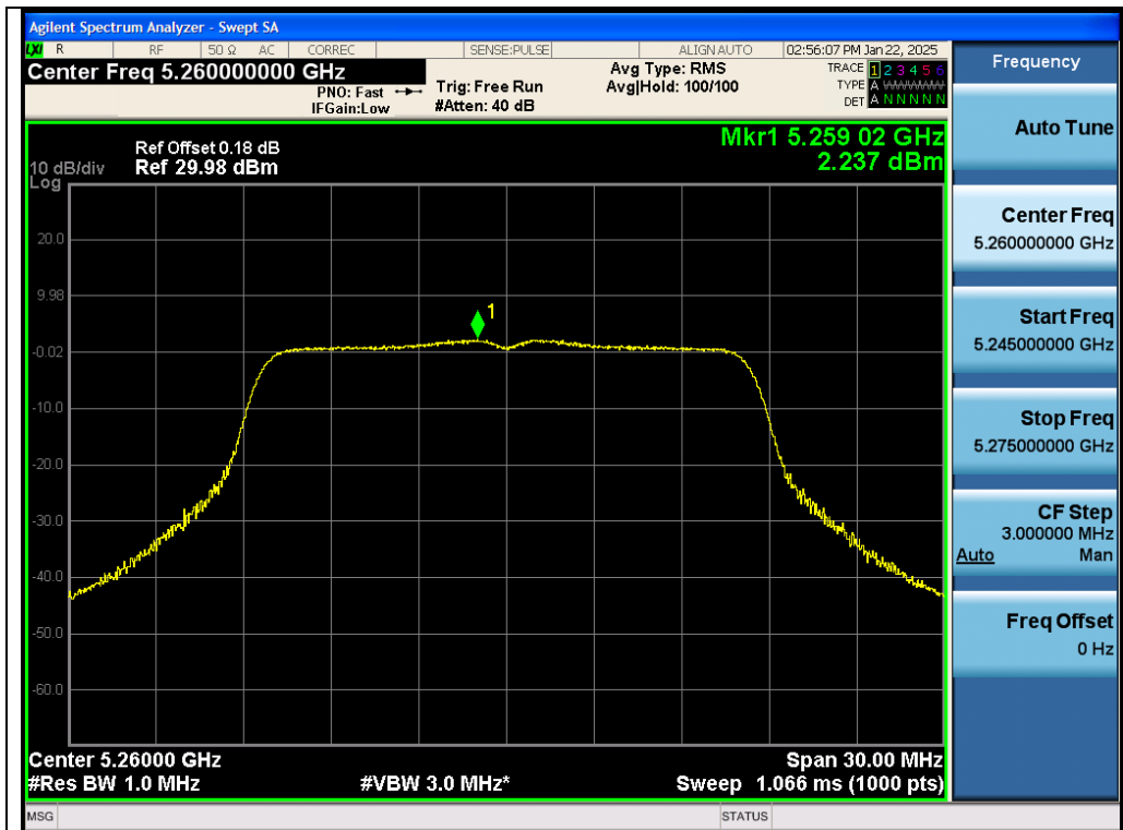
Test_Graph_802.11a_Chain A_5260_6Mbps_PSD
