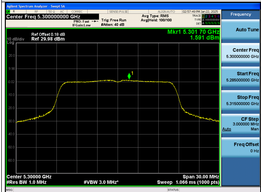
Test_Graph_802.11a_Chain A_5300_6Mbps_PSD
