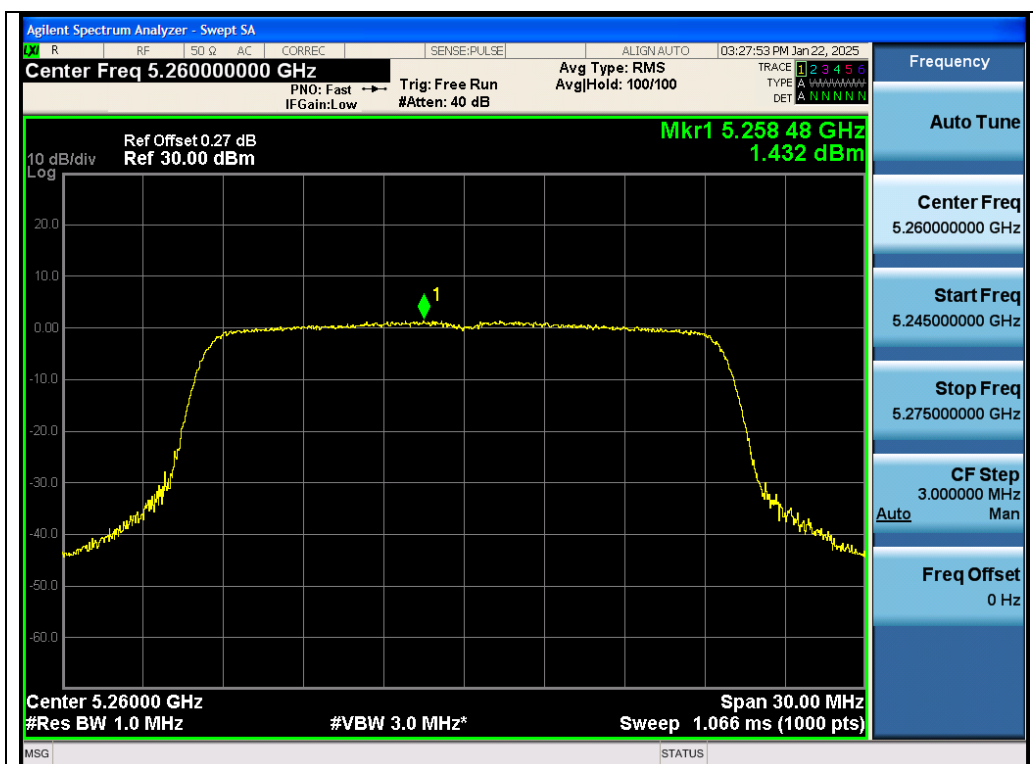
Test_Graph_802.11ax20_Chain A_5260_MCS0_PSD
