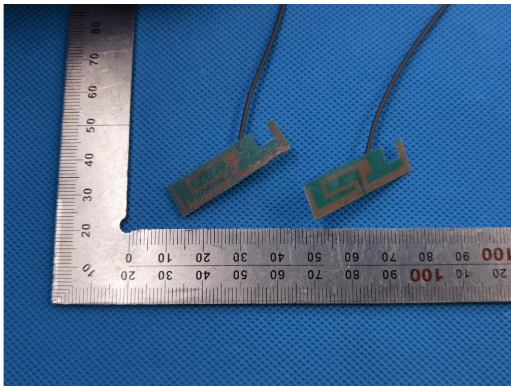
2.4G WLAN ANTENNA VIEW (FIGURE 2)
