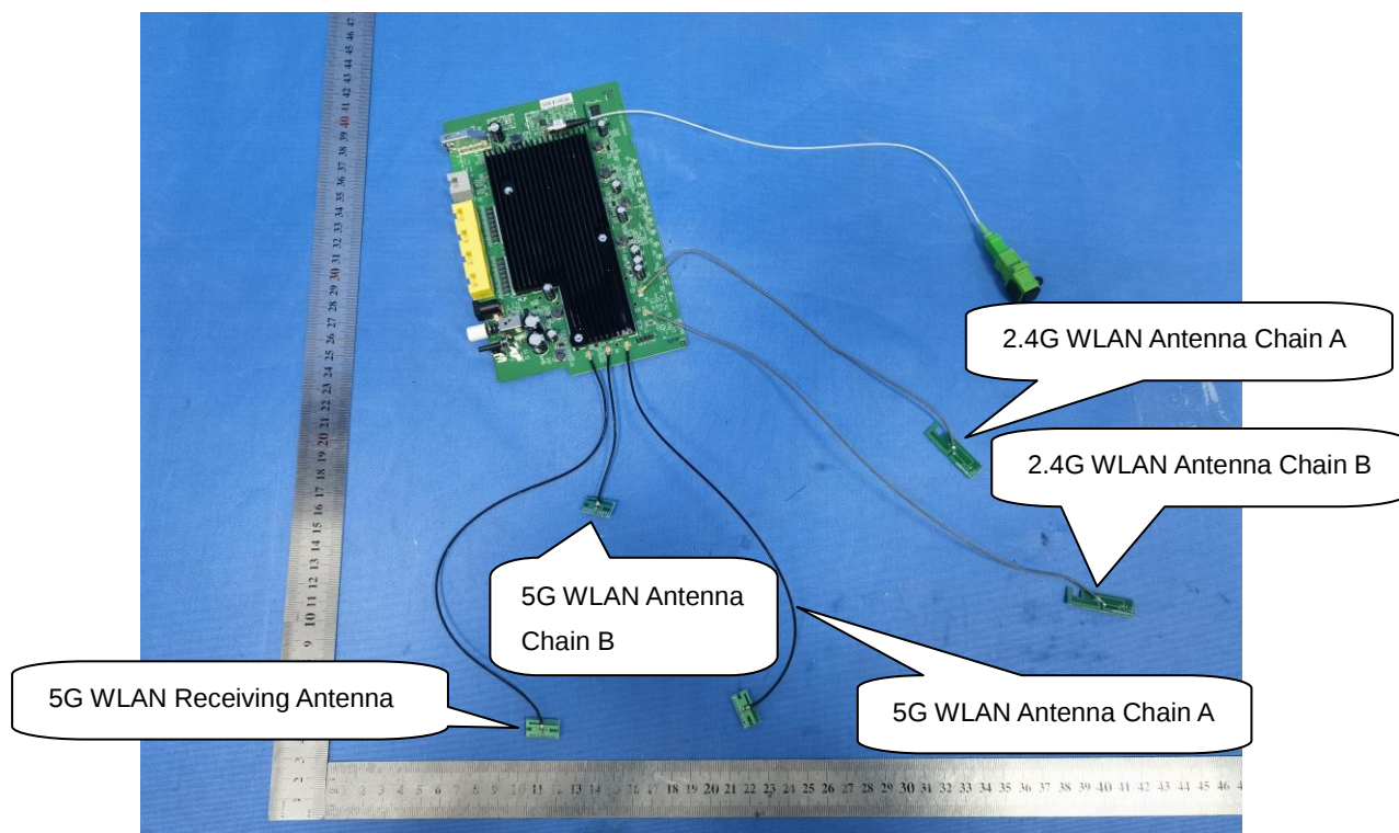
INTERNAL VIEW OF EUT (FIGURE 2)
