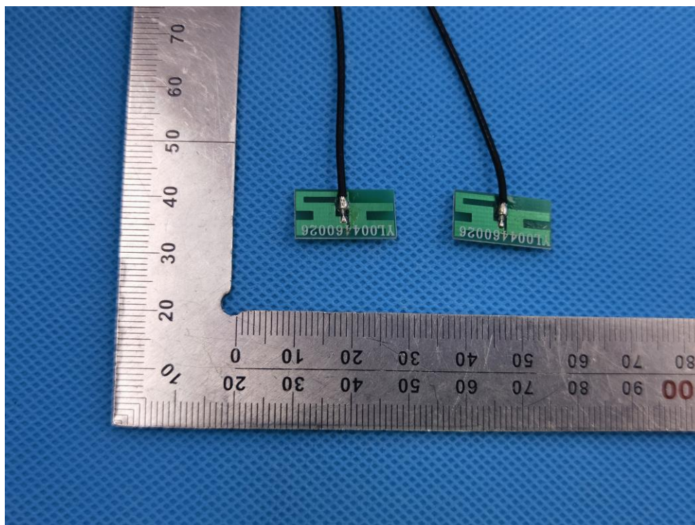
5G WLAN ANTENNA VIEW (FIGURE 2)
