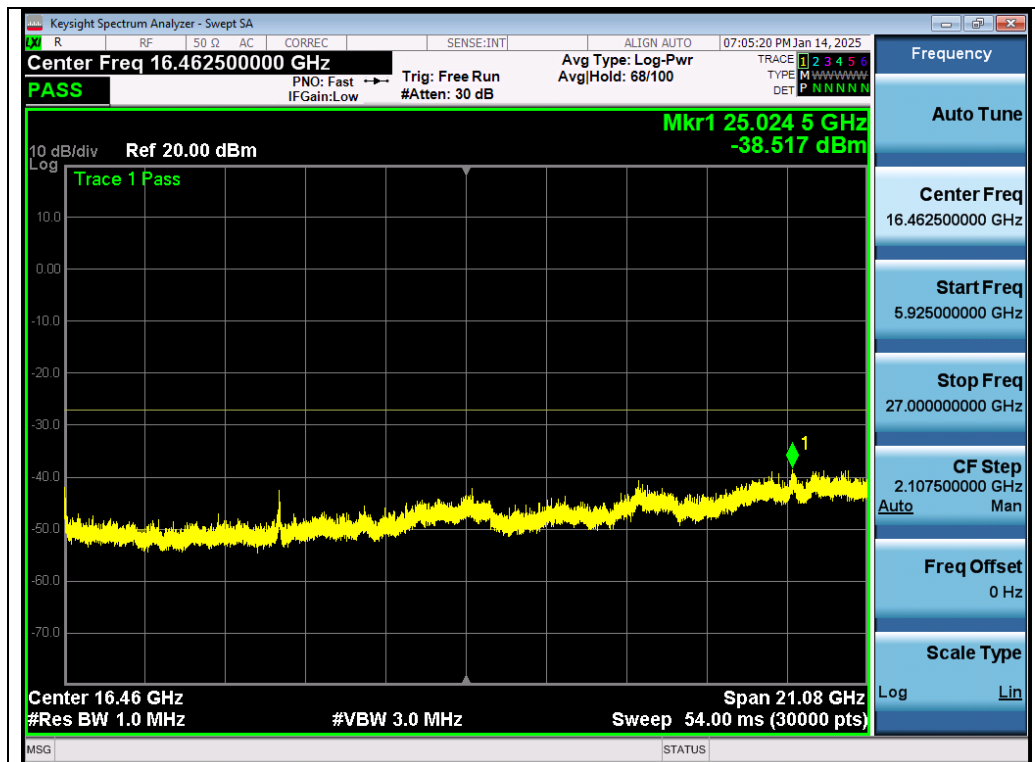
Test_Graph_802.11ax80_Chain A_5775_MCS0_Frequency Band4
