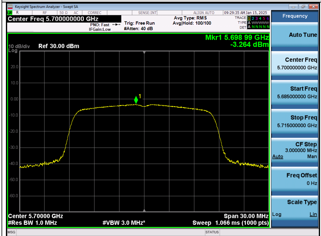
Test_Graph_802.11a_Chain B_5700_6Mbps_PSD
