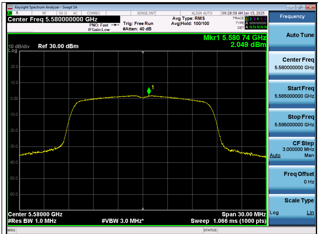
Test_Graph_802.11a_Chain B_5580_6Mbps_PSD
