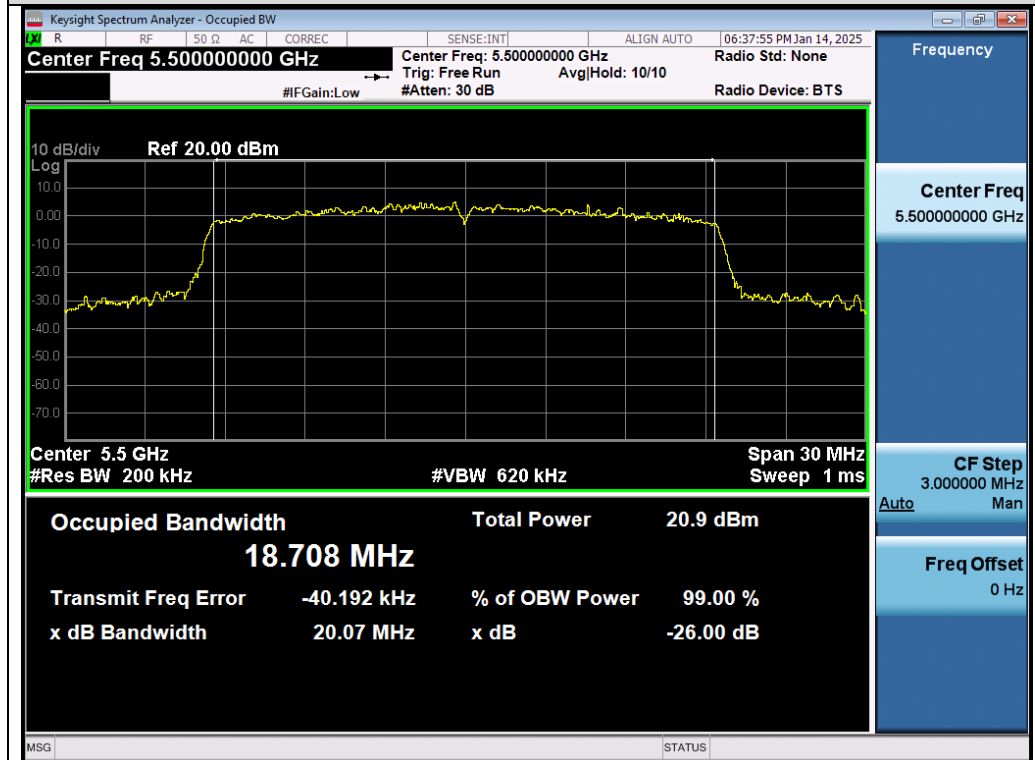
Test_Graph_802.11ax20_Chain A_5500_MCS0_OBW
