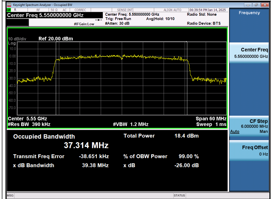
Test_Graph_802.11ax40_Chain A_5550_MCS0_OBW
