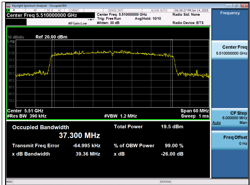
Test_Graph_802.11ax40_Chain A_5510_MCS0_OBW
