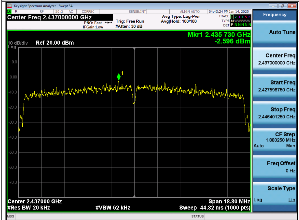
Test_Graph_802.11n20_Chain A_2437_MCS0_PSD
