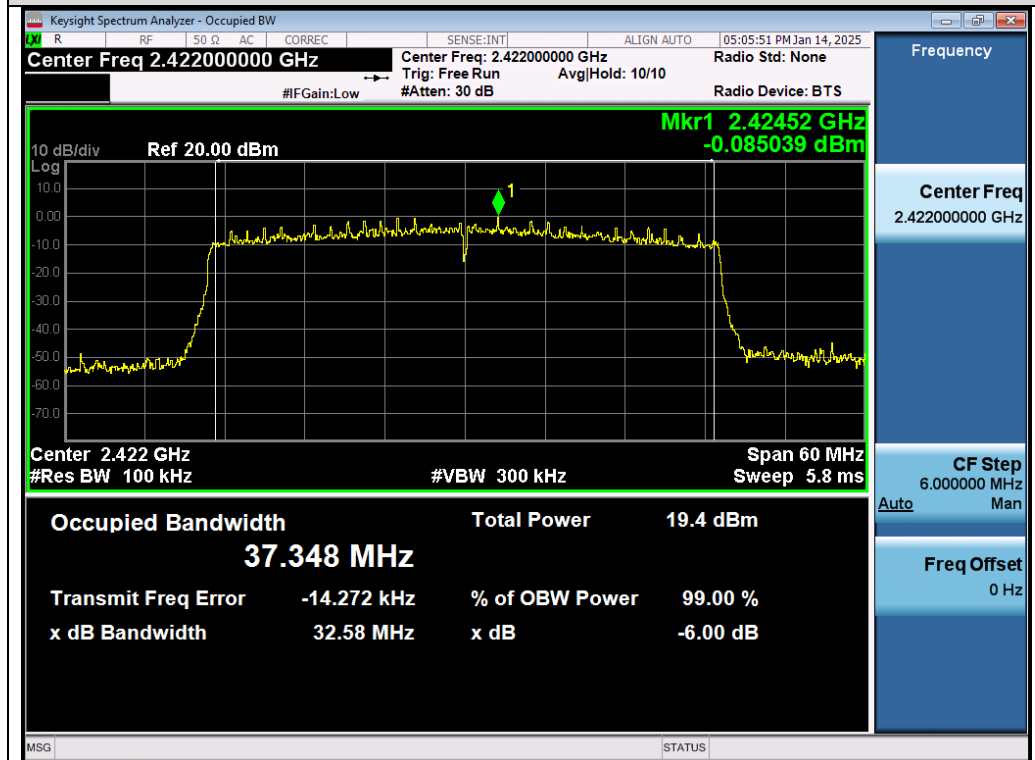
Test_Graph_802.11ax40_Chain A_2422_MCS0_DTSBW
