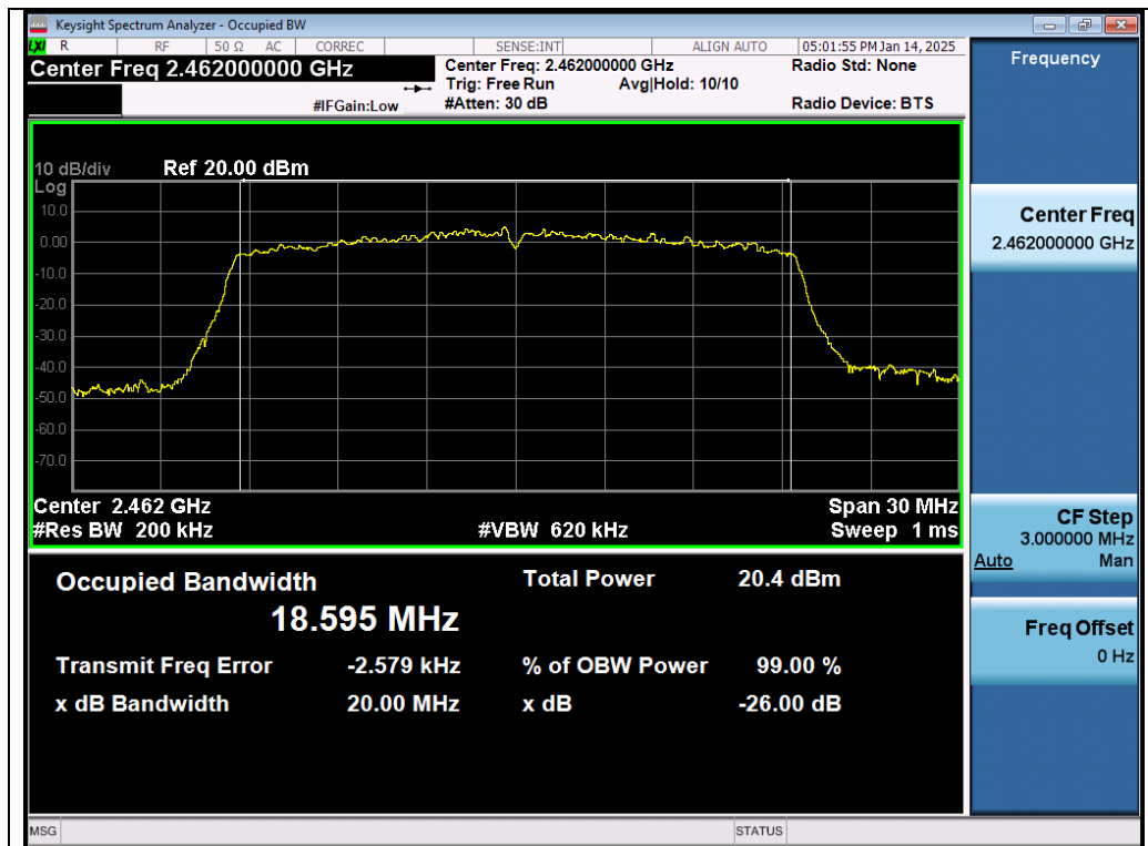
Test_Graph_802.11ax20_Chain A_2462_MCS0_OBW
