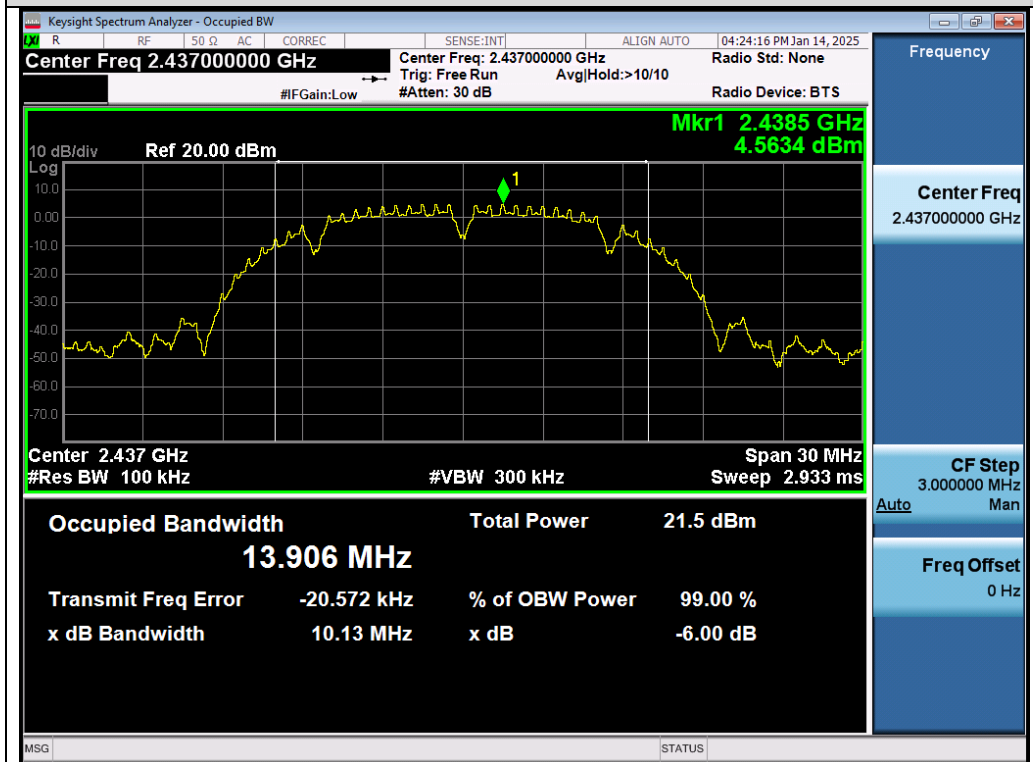
Test_Graph_802.11b_Chain A_2437_1Mbps_DTSBW
