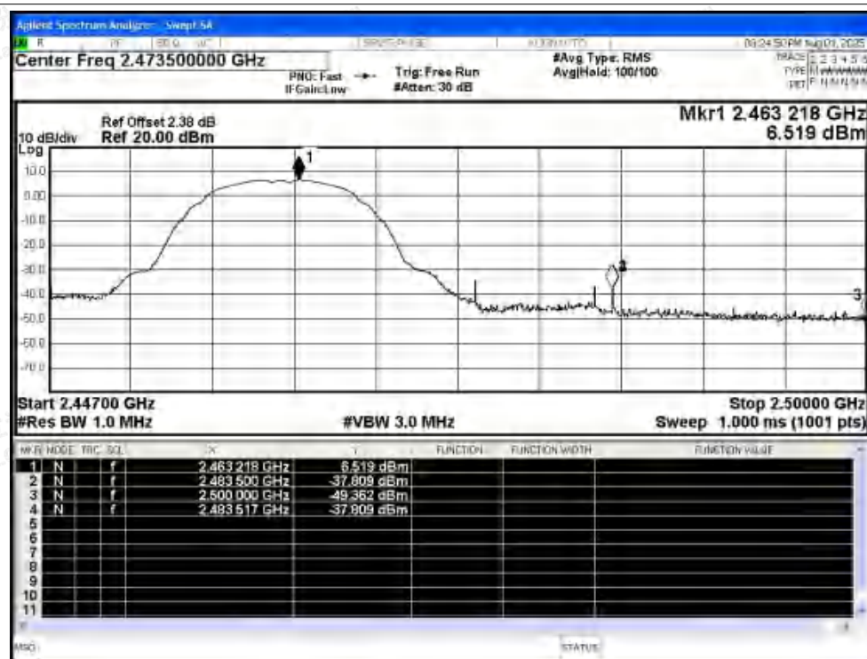
Restrict Band NVNT b 2462MHz Ant2 Average
