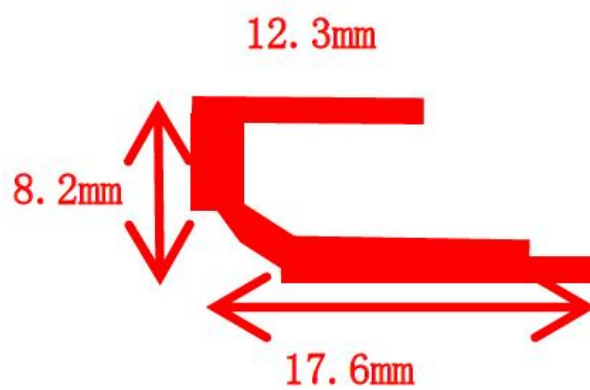
WIFI ANT 1
