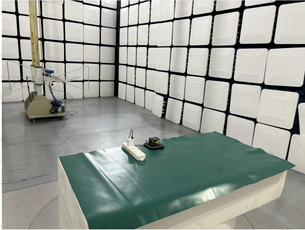
Photo of Radiation Emission Test (30MHz~1000MHz)
