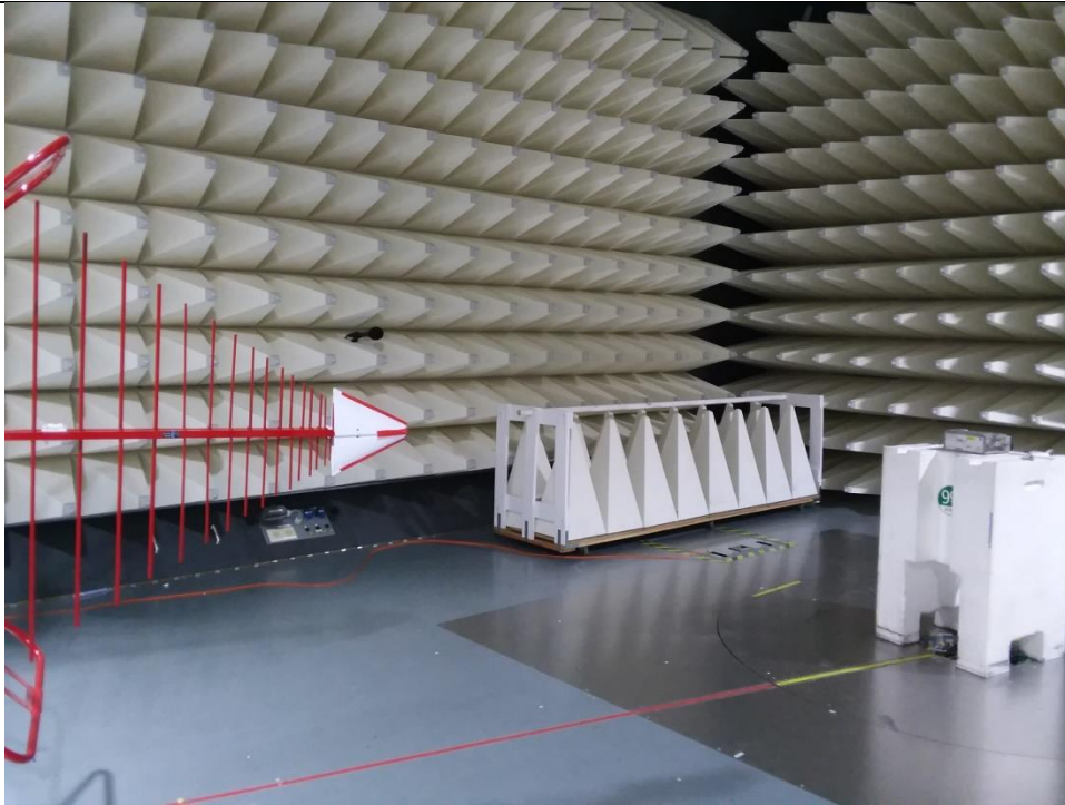
Figure C3. Radiated Emission Low Range test setup
