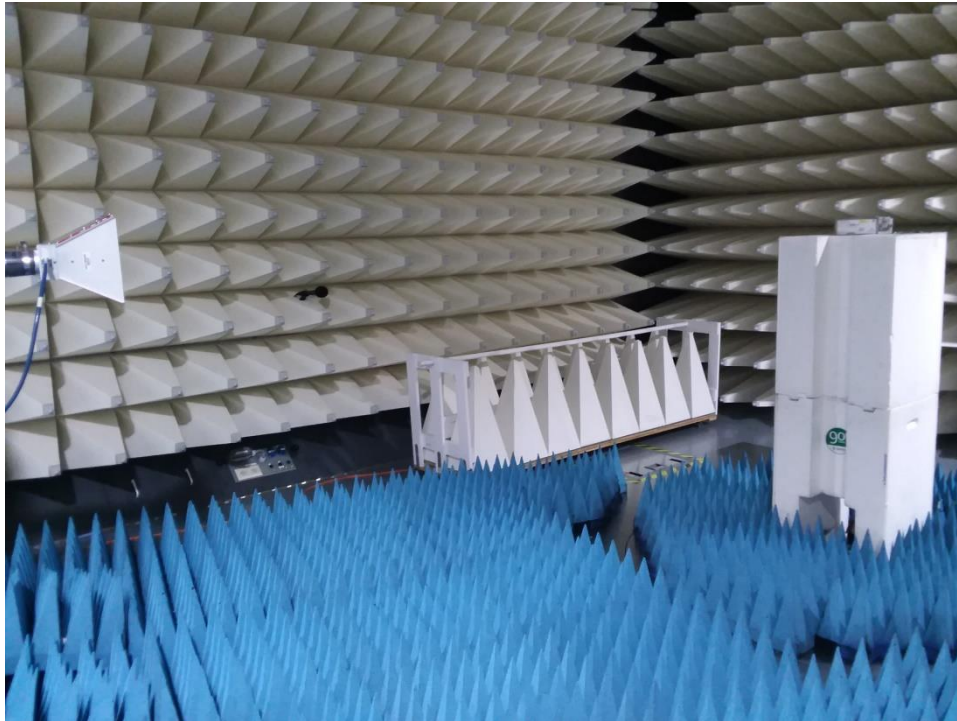
Figure C4. Radiated Emission High Range 1-18GHz test setup 1-18GHz test setup
