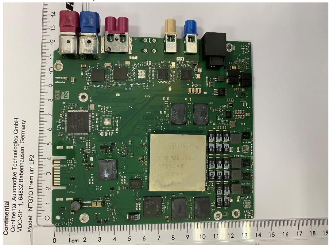
Multimedia board 2.6 top view
