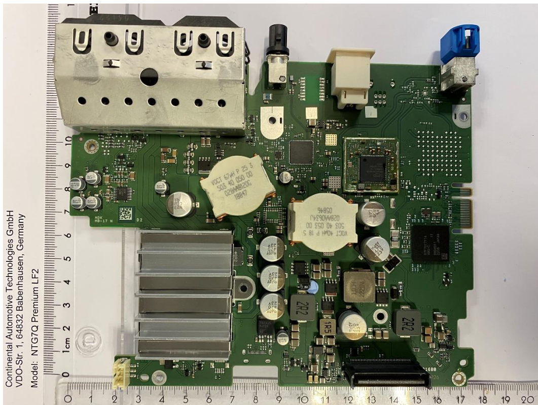
Base board 4 Wi-Fi module without shield
