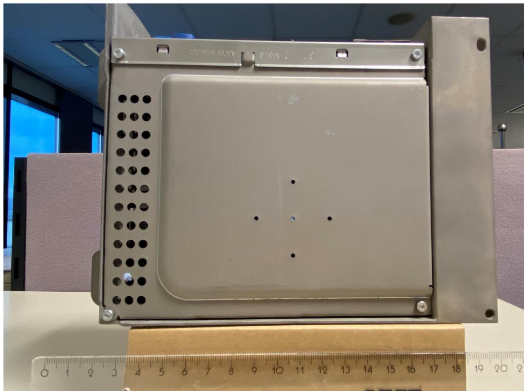
Bottom view
