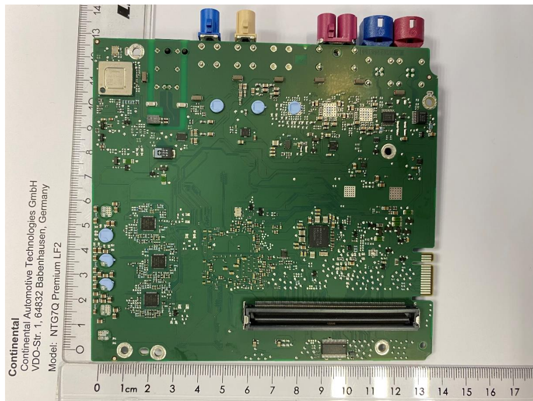
Multimedia board 2.6 bottom view
