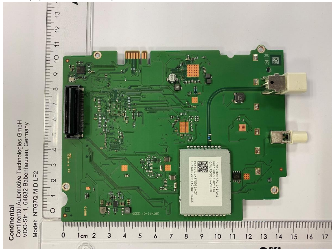
Country specific board 4.2 top view with shield
