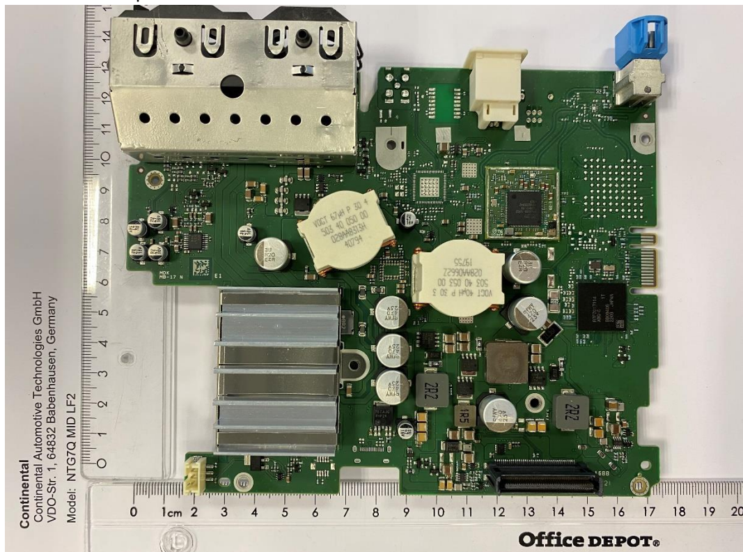
Base board 6 top view Wi-Fi module without shield
