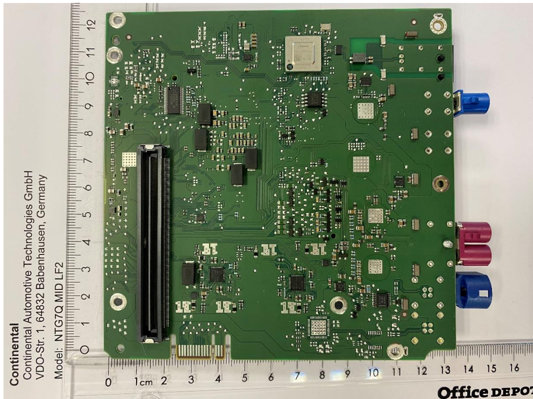
Multimedia board 1.4 bottom view
