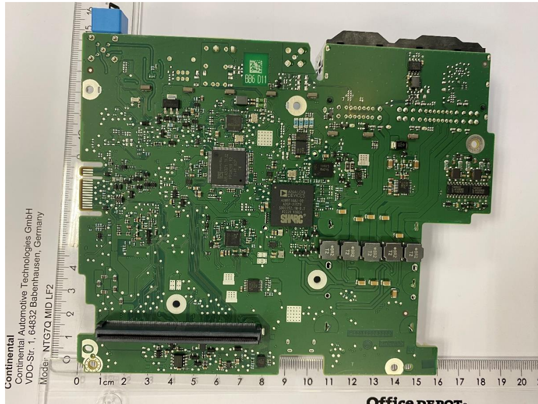
Base board 6 bottom view
