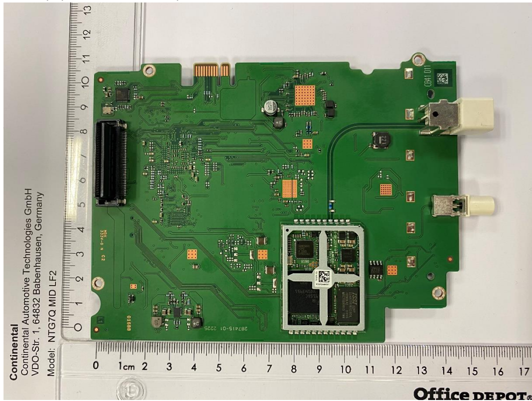
Country specific board 4.2 top view without shield
