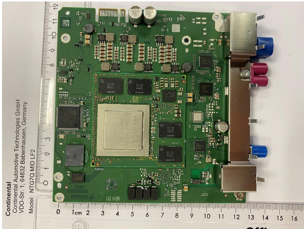
Multimedia board 1.4 top view
