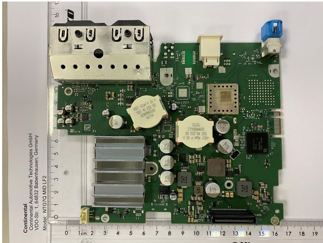
Base board 6 top view Wi-Fi module with shield
