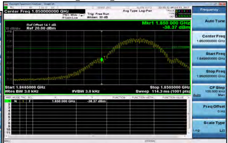
GPRS_1900MHz_LowCH512-1850.2
