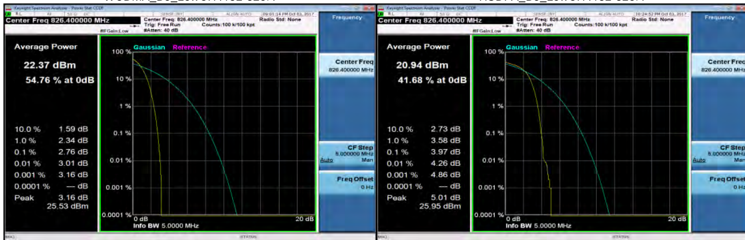
WCDMA_B5_LowCH4132-826.4
