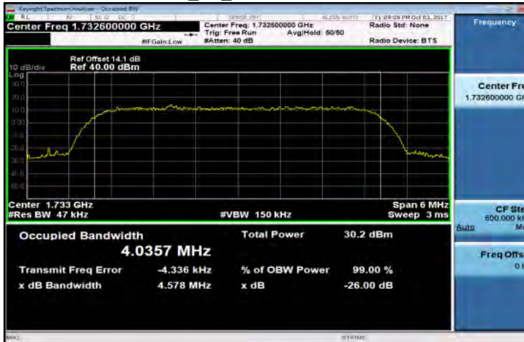
HSDPA_B4_MidCH1413-1732.6
