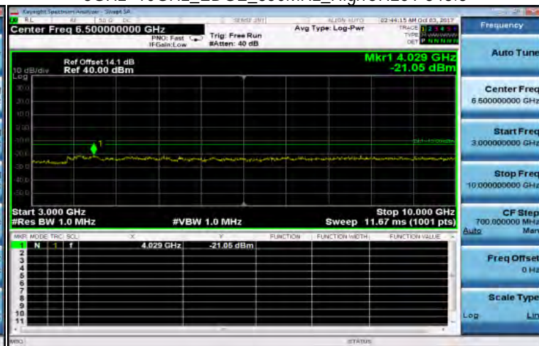
3GHz~10GHz_EDGE_850MHz_HighCH251-848.8
