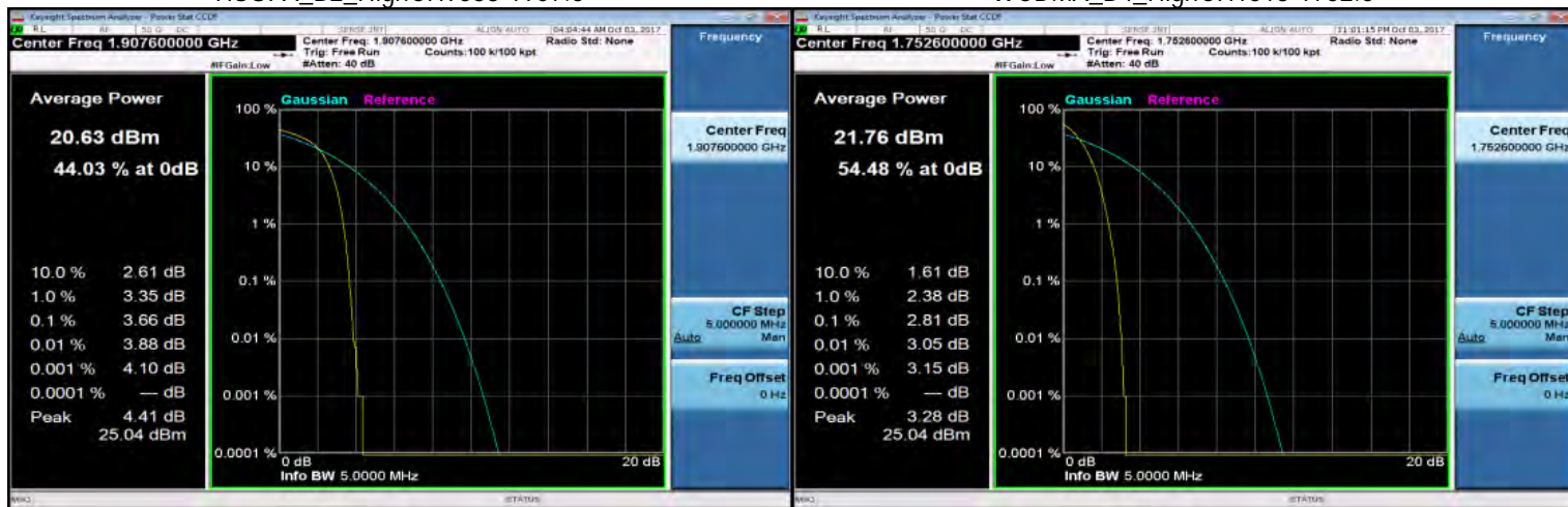
HSUPA_B2_HighCH9538-1907.6
