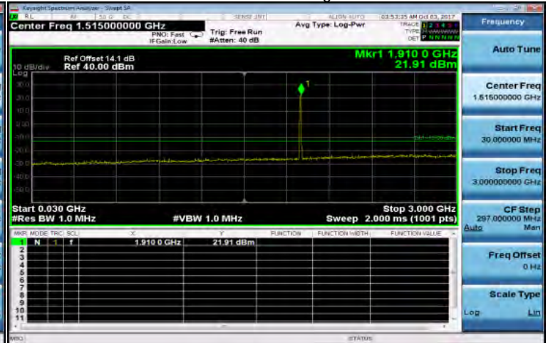
30MHz~3GHz_HSDPA_B2_HighCH9538-1907.6
