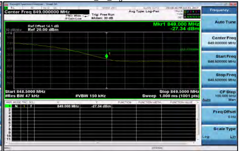
WCDMA_B5_HighCH4233-846.6
