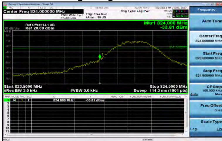
EDGE_850MHz_LowCH128-824.2
