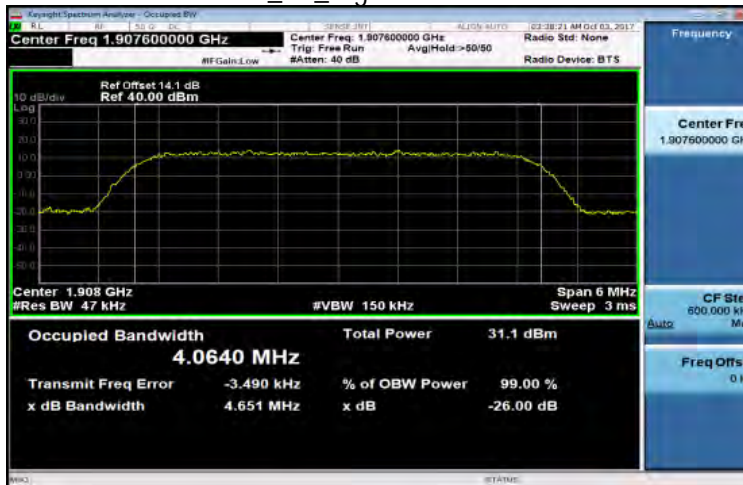
WCDMA_B2_HighCH9538-1907.6
