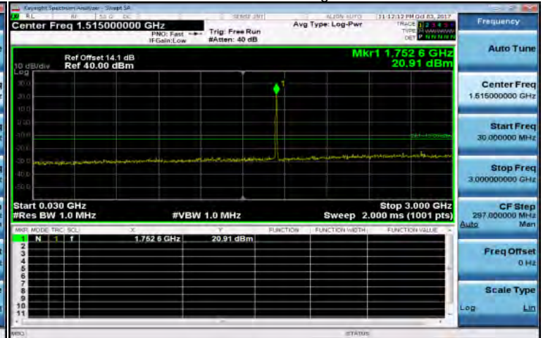
30MHz~3GHz_HSDPA_B4_HighCH1513-1752.6
