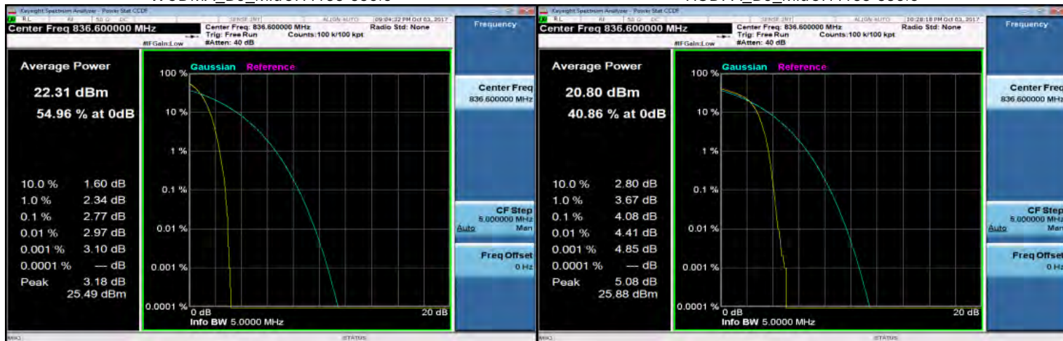
WCDMA_B5_MidCH4183-836.6
