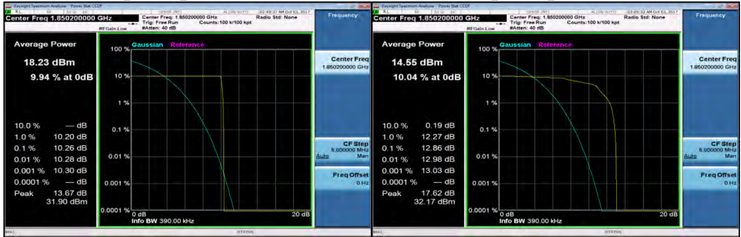
GPRS_1900MHz_LowCH512-1850.2
