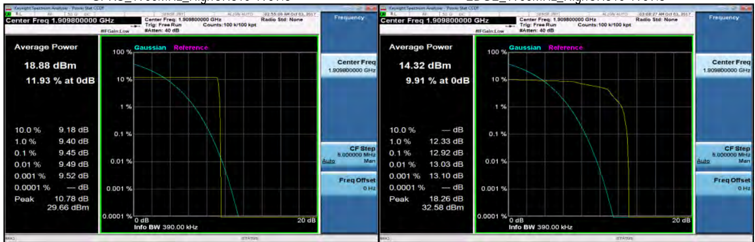
GPRS_1900MHz_HighCH810-1909.8
