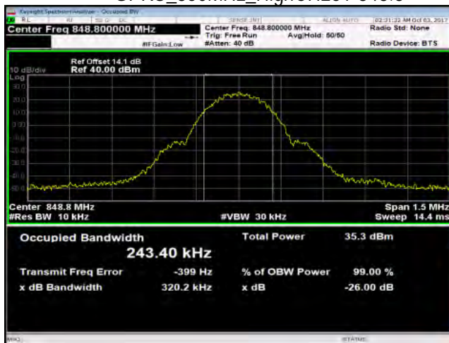
GP RS_850MHz_HighCH251-848.8
