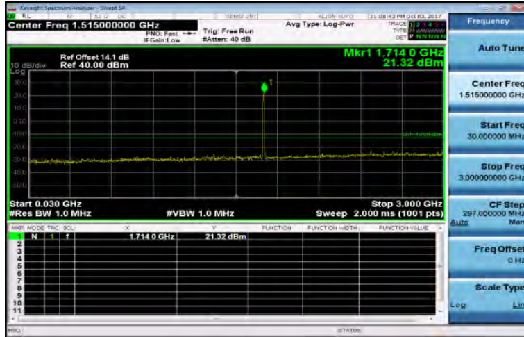
30MHz~3GHz_HSDPA_B4_LowCH1312-1712.4
