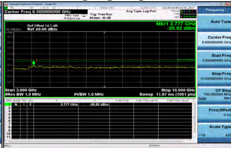
3GHz~10GHz_EDGE_850MHz_MidCH190-836.6
