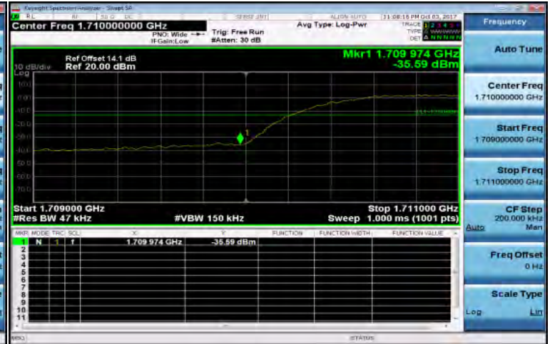
HSDPA_B4_LowCH1312-1712.4
