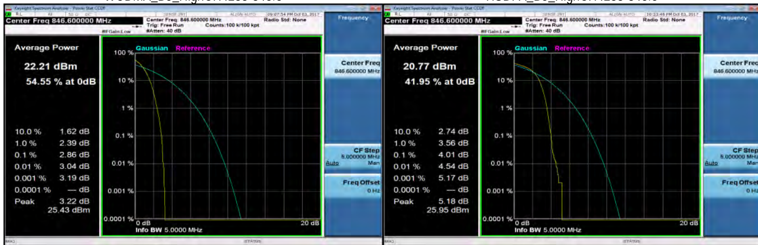
WCDMA_B5_HighCH4233-846.6
