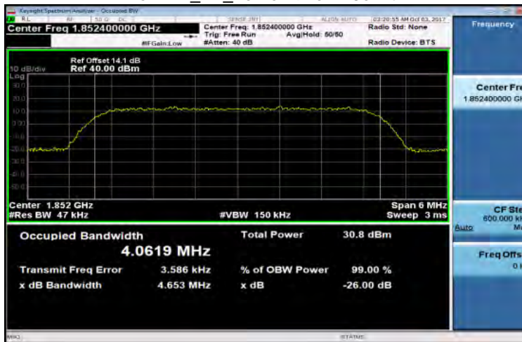
WCDMA_B2_LowCH9262-1852.4
