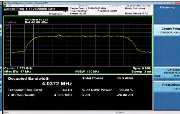
HSUPA_B4_MidCH1413-1732.6
