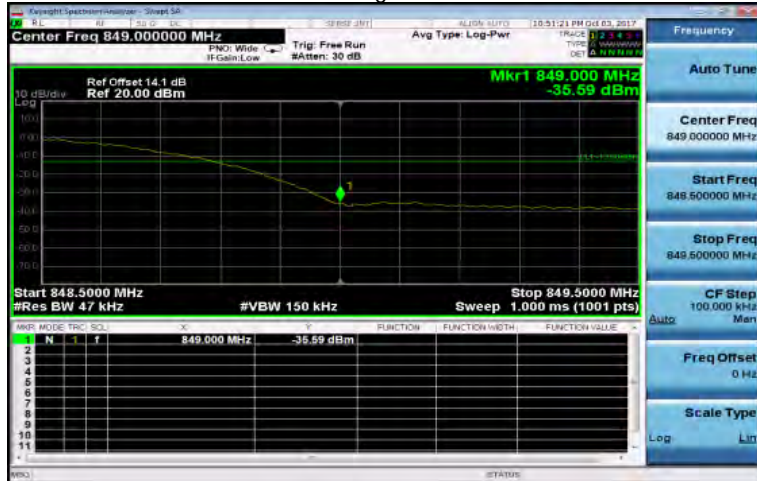
HSUPA_B5_HighCH4233-846.6
