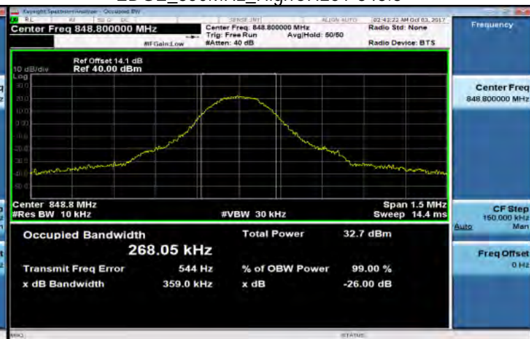
EDGE_850MHz_HighCH251-848.8
