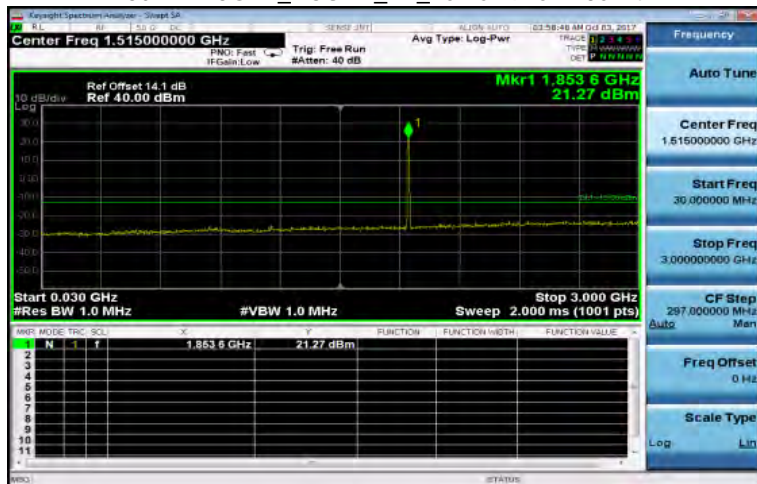
30MHz~3GHz_HSUPA_B2_LowCH9262-1852.4
