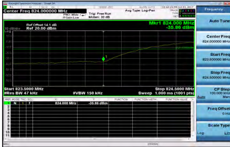
HSUPA_B5_LowCH4132-826.4
