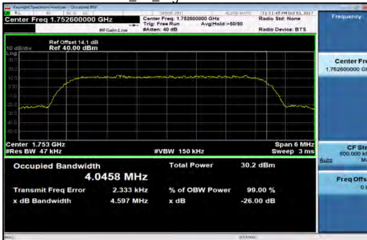
HSDPA_B4_HighCH1513-1752.6
