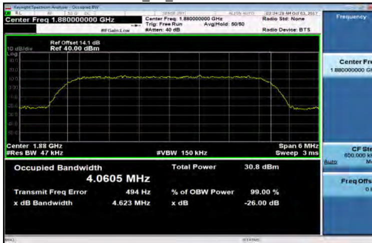
WCDMA_B2_MidCH9400-1880
