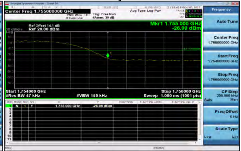
WCDMA_B4_HighCH1513-1752.6
