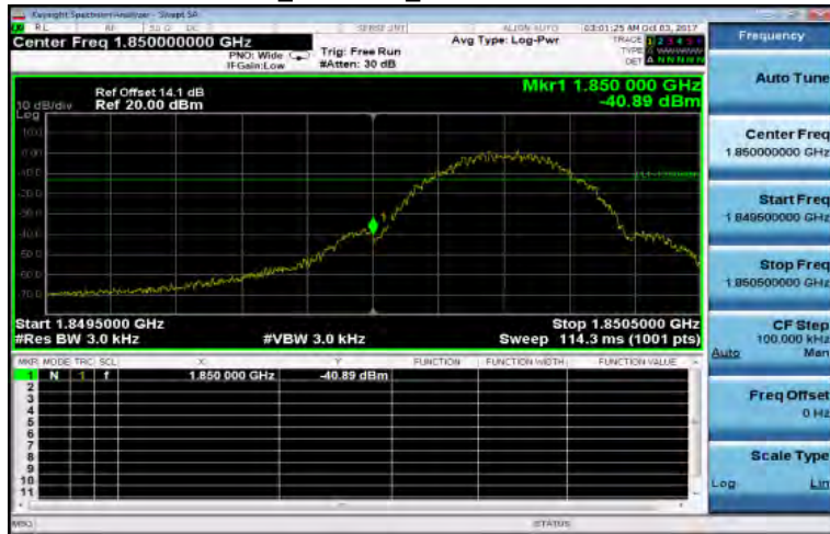
EDGE_1900MHz_LowCH512-1850.2
