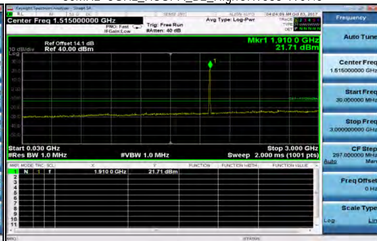
30MHz~3GHz_HSUPA_B2_HighCH9538-1907.6
