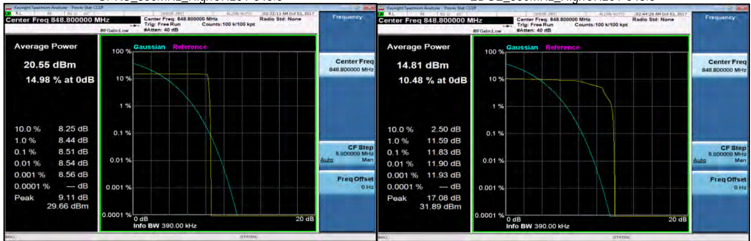
GPRS_850MHz_HighCH251-848.8
