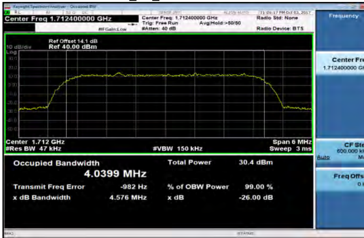
HSDPA_B4_LowCH1312-1712.4
