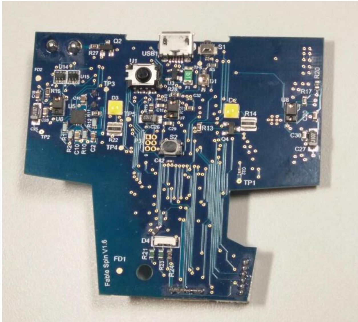
Figure 2 - Spin Module PCB Bottom Side
