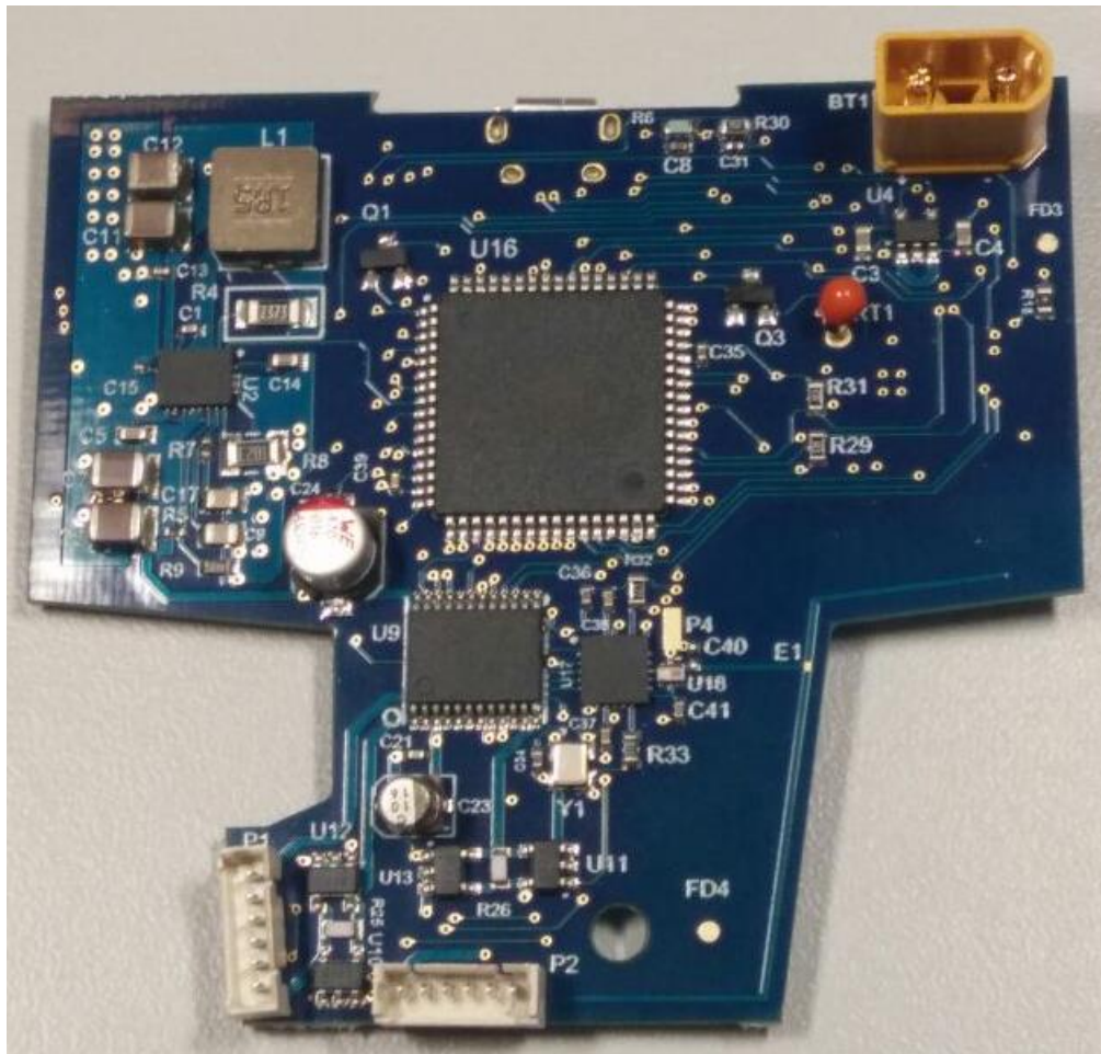
Figure 1 - Spin Module Top Side
