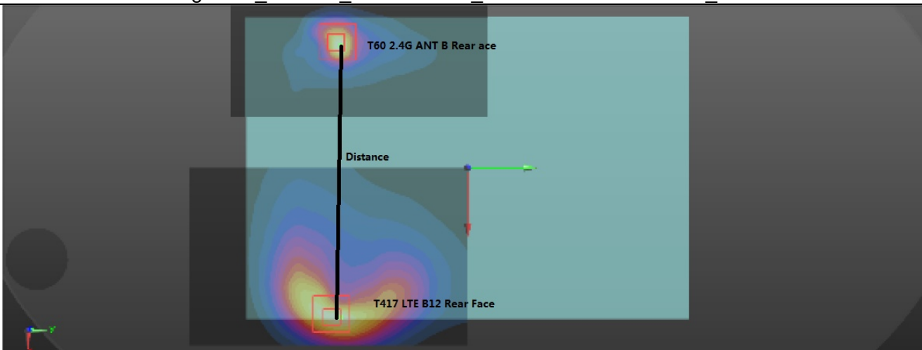
Fig9 T60_802.11b_Ant B + T417_LTE B12 with Rear Face_0cm
