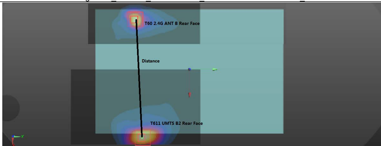
Fig5 T60_802.11b_Ant B + T633_UMTS B4 with Rear Face_0cm
