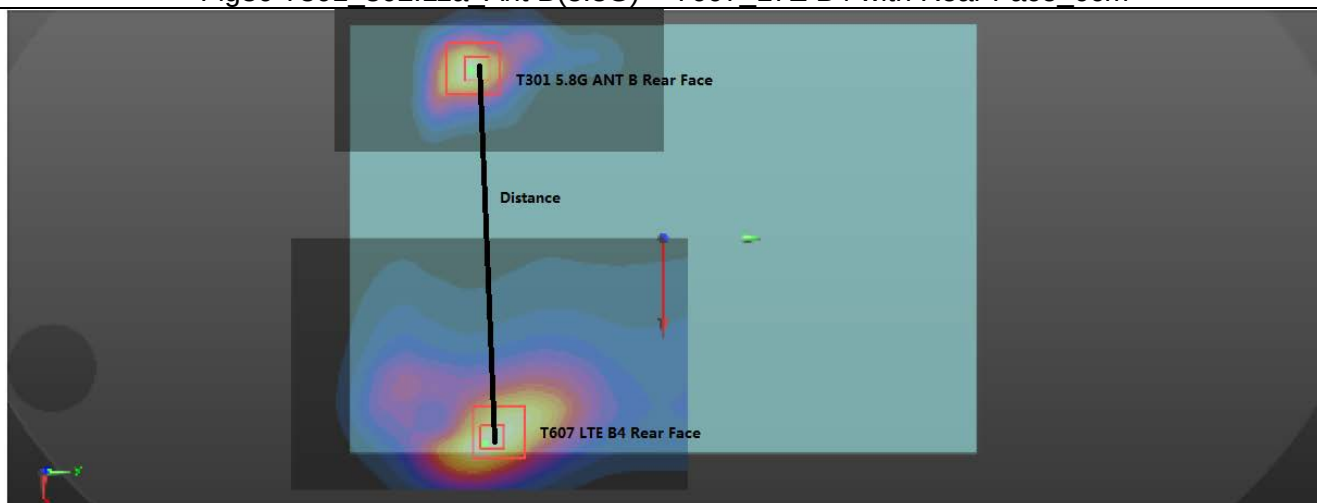
Fig30 T301_ 802.11a Ant B(5.8G) + T607_ LTE B4 with Rear Face_ 0cm
