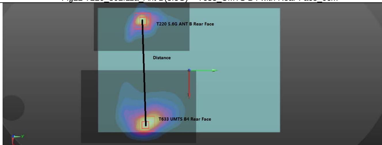
Fig23 T220_802.11a_Ant B(5.5G) + T655_UMTS B5 with Rear Face_0cm
