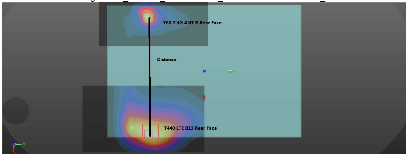
Fig11 T60_ 802.11b Ant B + T470_LTE B25 with Rear Face_0cm
