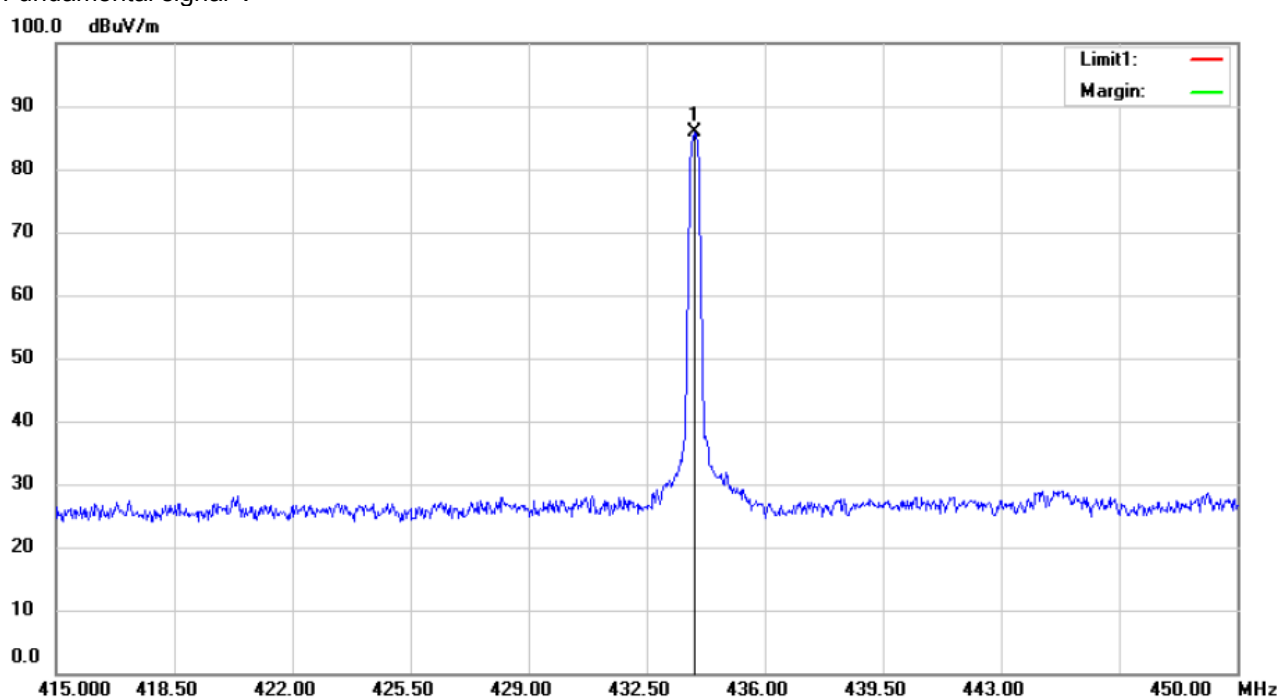
Fundamental signal-V
