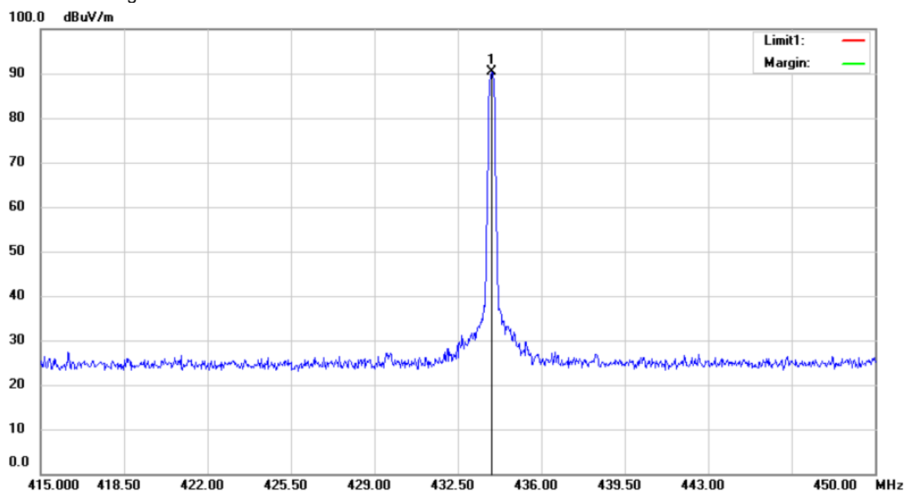
Fundamental signal-V
