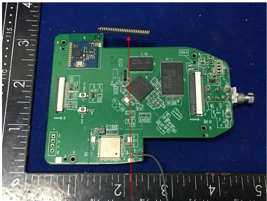
433MHz receiver antenna
