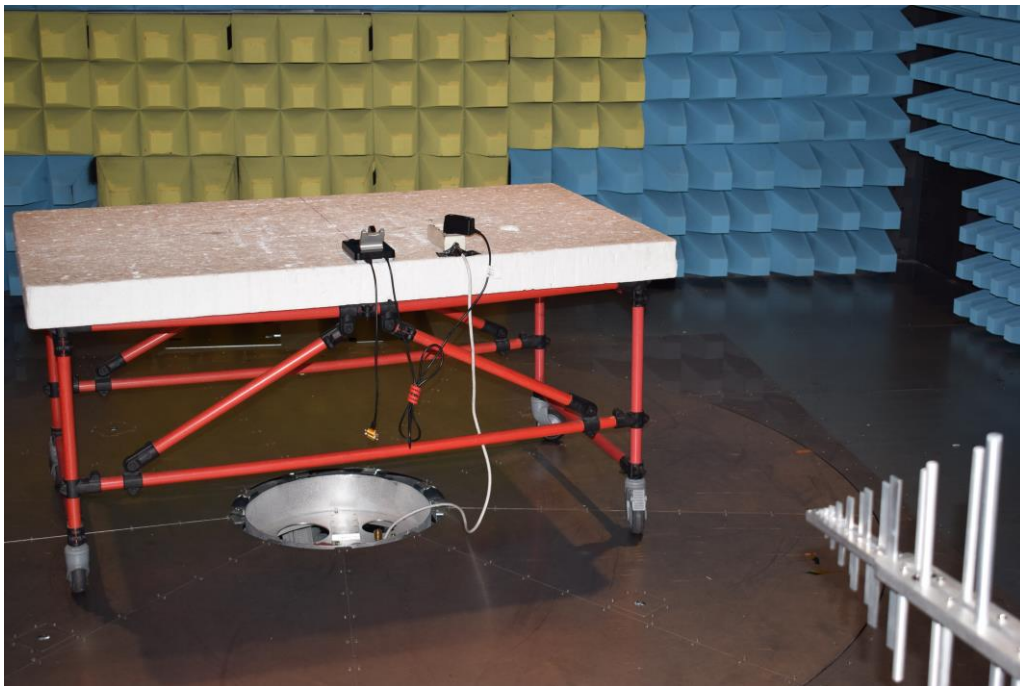
Picture 6: SAC, radiated emission test 30 MHz – 1 GHz – Standby (rear view)
