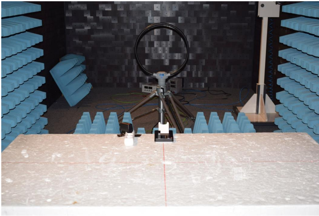
Picture 1: CDC, radiated emission test 9 kHz -30 MHz - Standby (front view)
