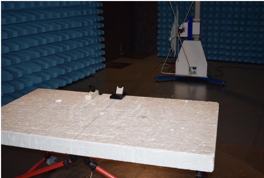
Picture 5: SAC, radiated emission test 30 MHz – 1 GHz – Standby (front view)
