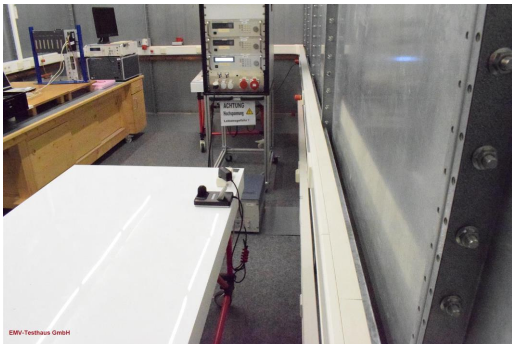
Picture 10: AC power line conducted emission – Standby (rear view)
