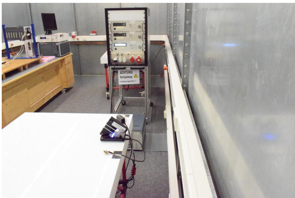
Picture 12: AC power line conducted emission – Charging (rear view)
