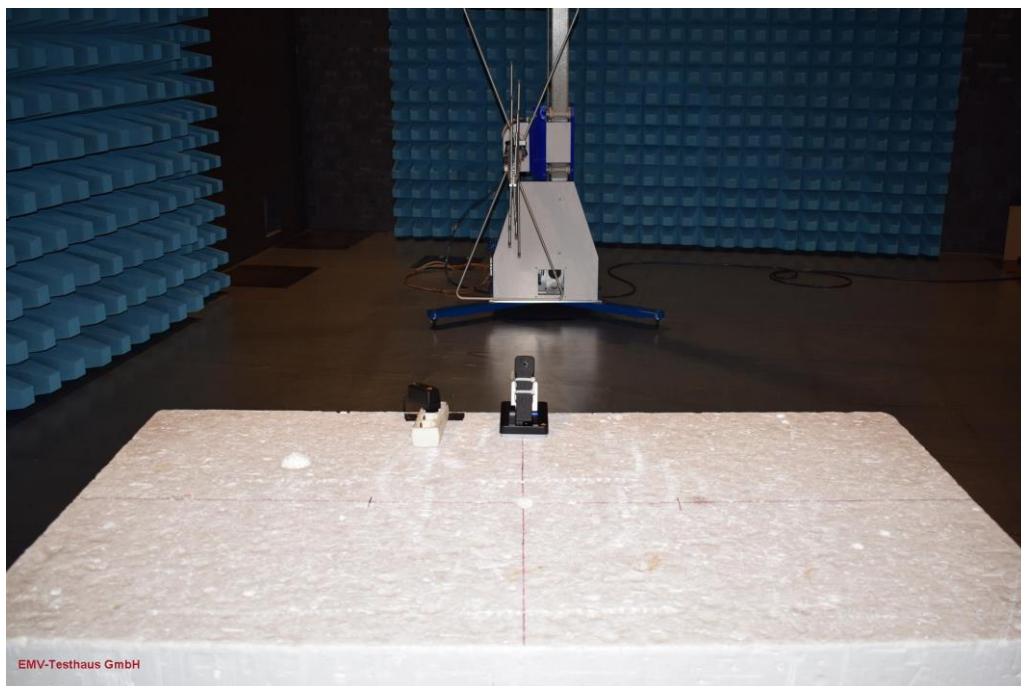
Picture 7: SAC, radiated emission test 30 MHz – 1 GHz – Charging (front view)
