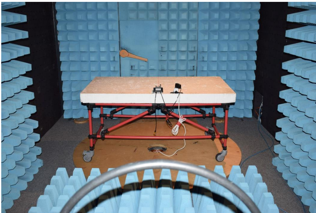
Picture 2: CDC, radiated emission test 9 kHz -30 MHz - Standby (rear view)
