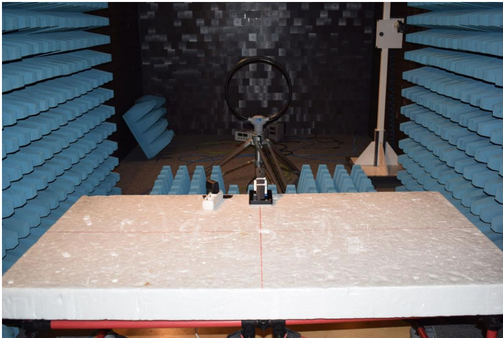
Picture 3: CDC, radiated emission test 9 kHz -30 MHz - Charging (front view)
