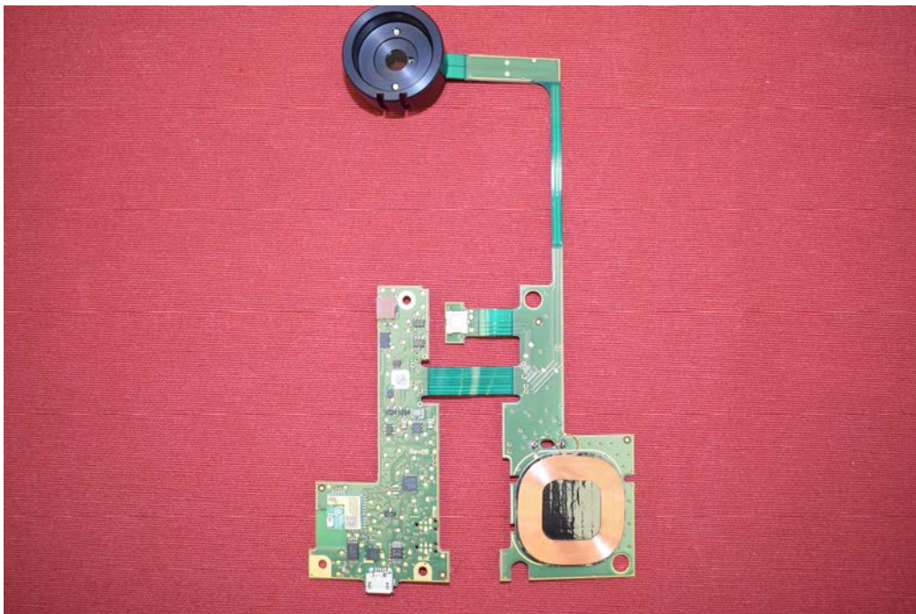
Picture 8: Peripheral device power receiver – PCB, bottom side
