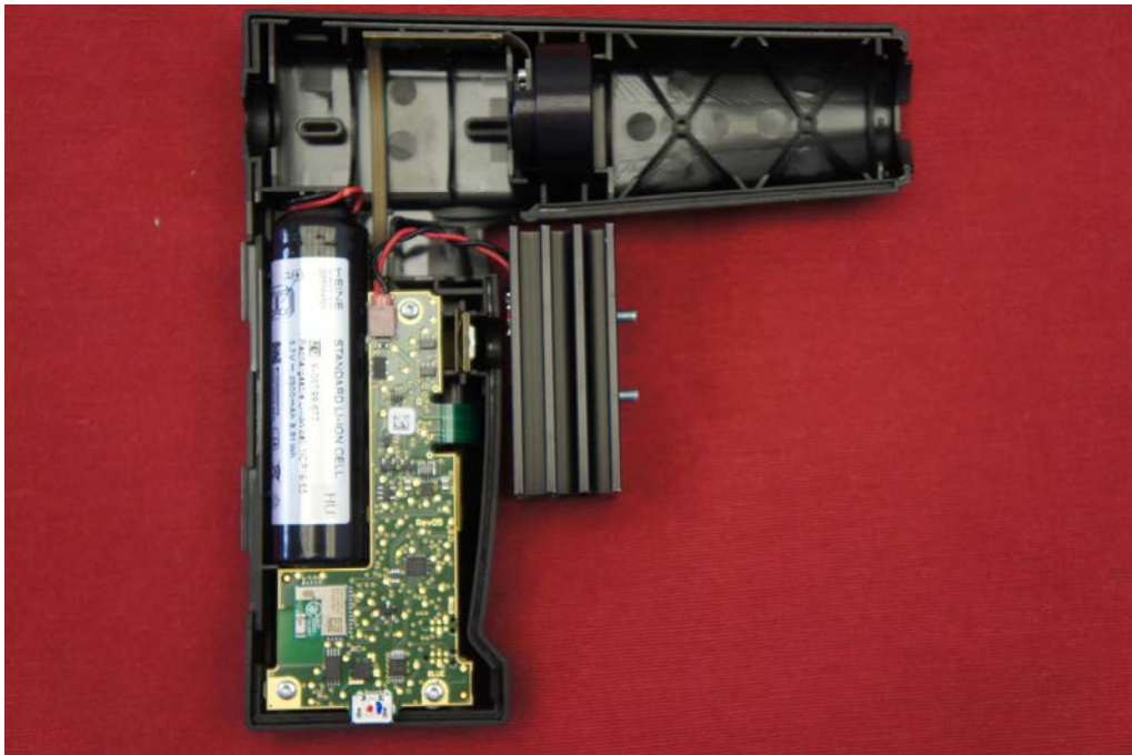
Picture 19: Peripheral device power receiver dummy – Open, top side
