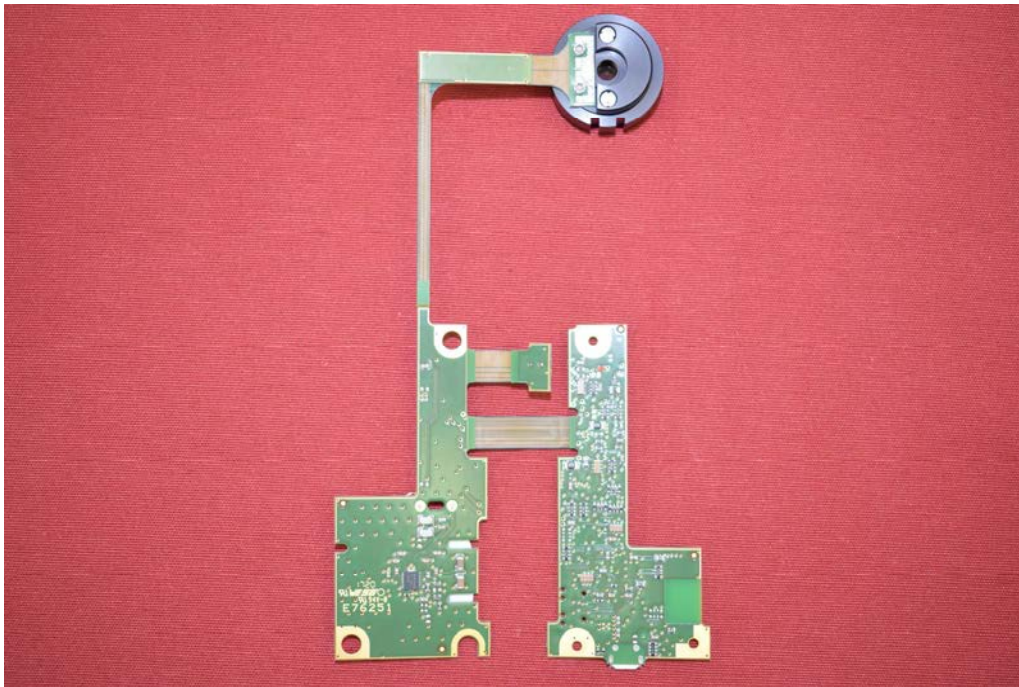
Picture 7: Peripheral device power receiver – PCB, top side
