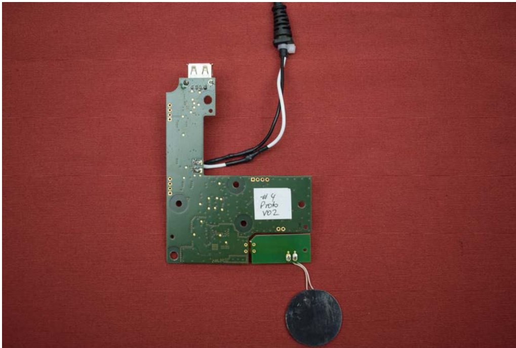
Picture 5: EUT power transmitter – PCB, bottom side
