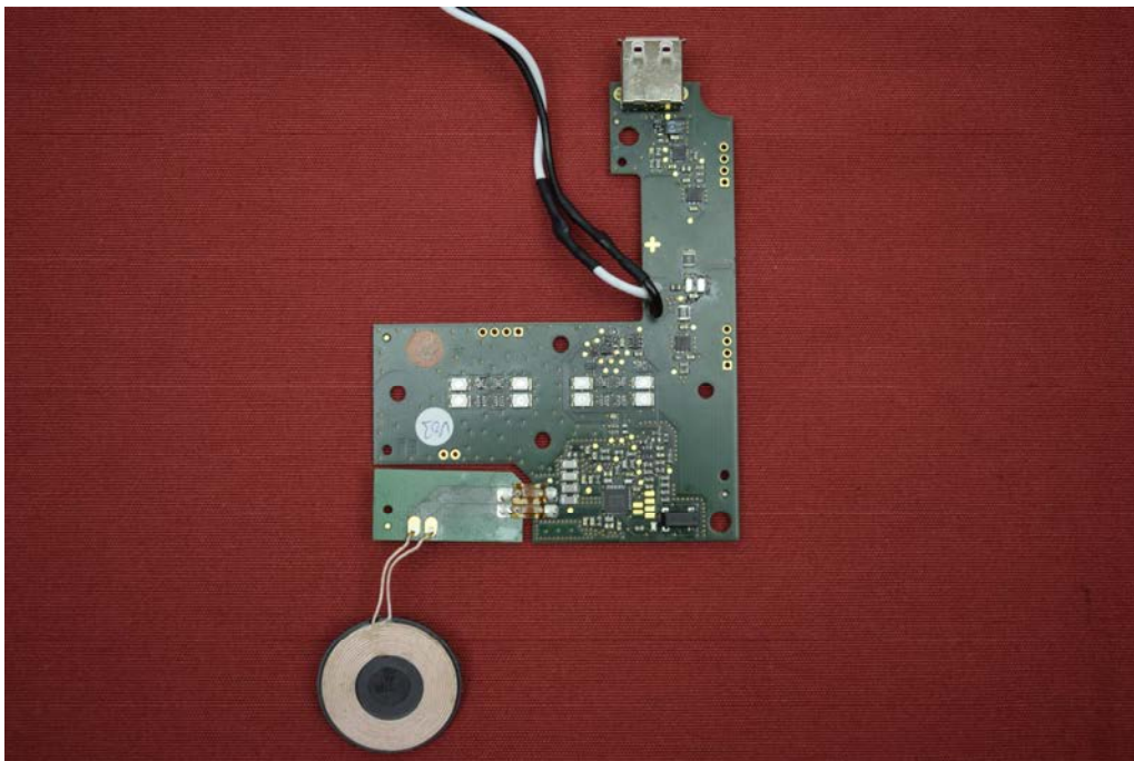
Picture 4: EUT power transmitter – PCB, top side
