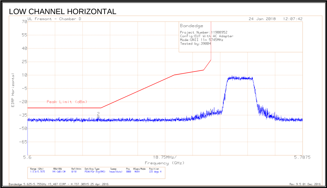
Trace Markers
