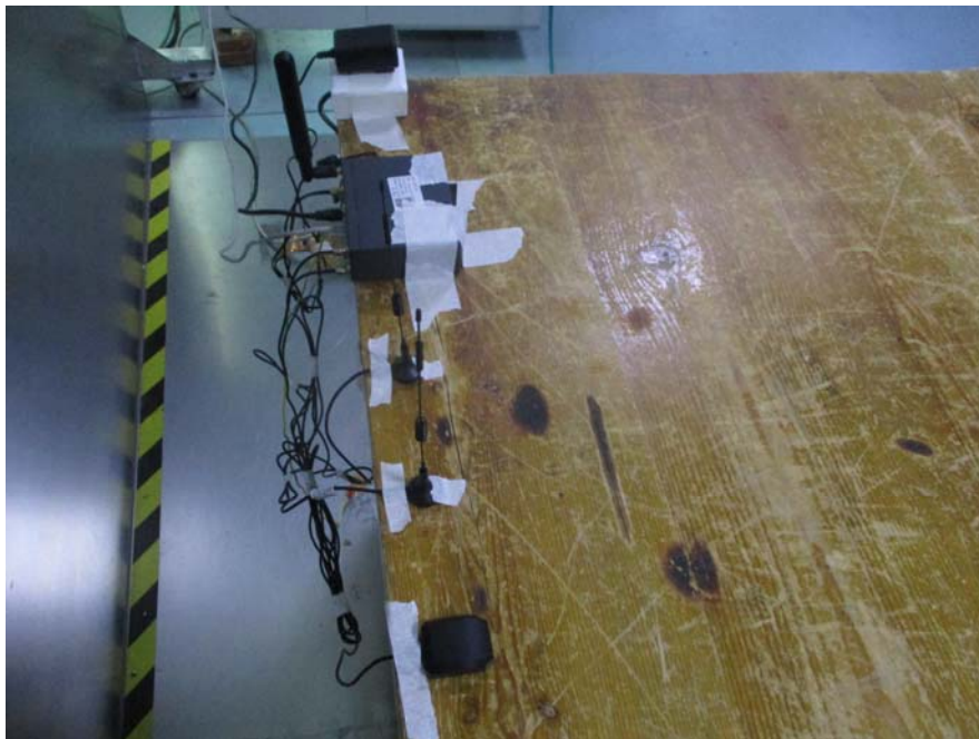
Conducted Emissions – Side View For UR52
