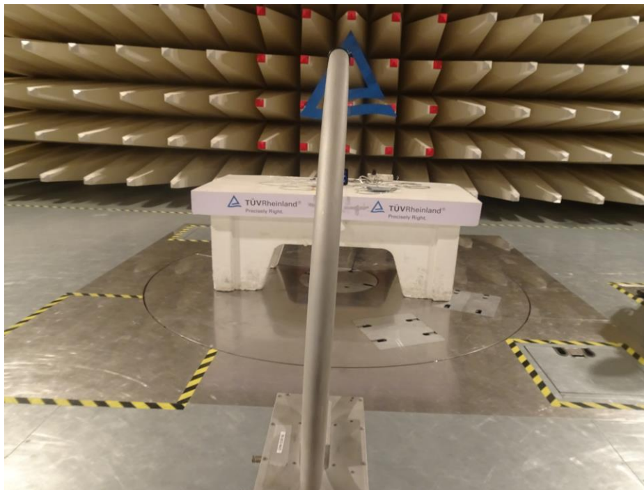
Test setup Frequency Range 9kHz-30MHz Active Loop Antenna
