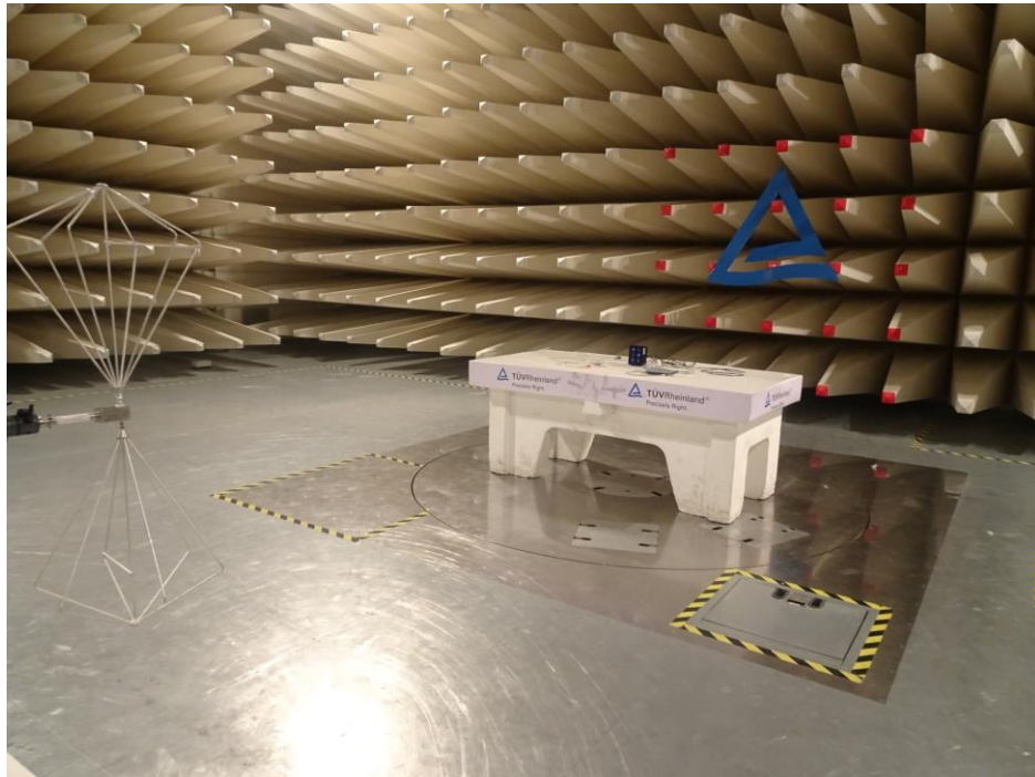
Test setup Frequency Range 30MHz-200MHz Biconical Antenna
