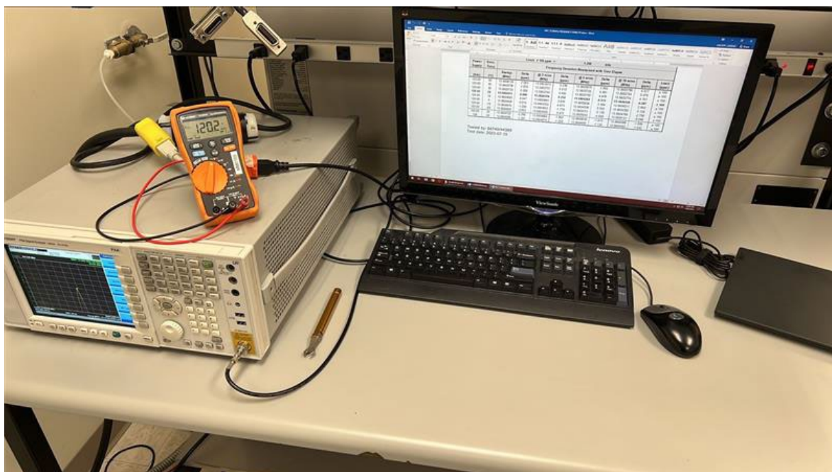
CONDUCTED TEST EQUIPMENT SETUP
