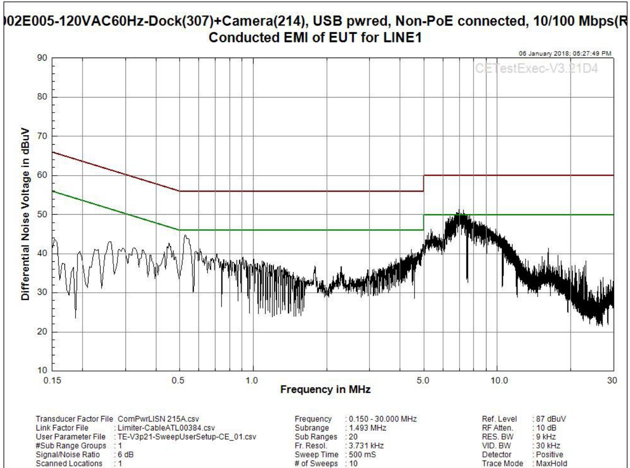
Figure 6.14 - Conducted Emission Scan Line 1 (Line L)
