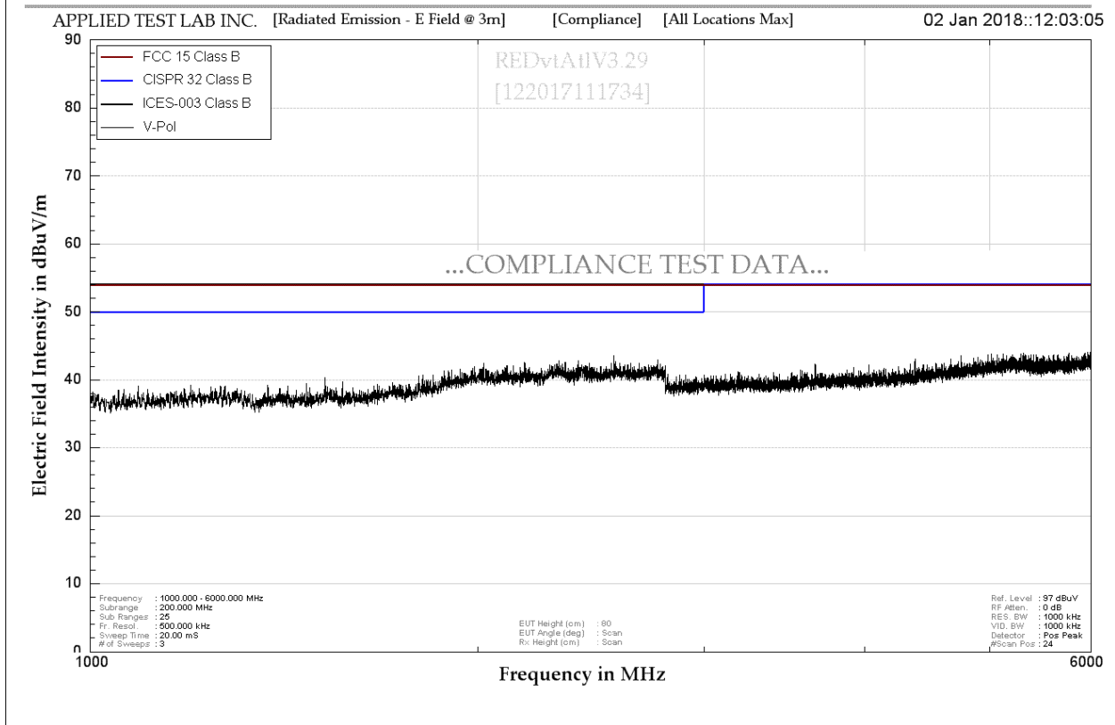
Figure 6.6 - Radiated Emission (FCC) - Scan Vertical Polarization (1000MHz - 6000MHz)
