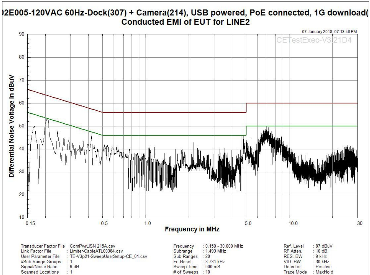
Figure 6.17 - Conducted Emission Scan Line 2 (Line N)
