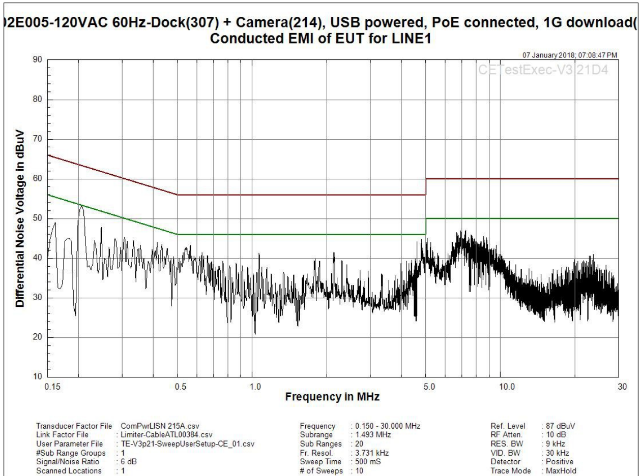
Figure 6.16 - Conducted Emission Scan Line 1 (Line L)
