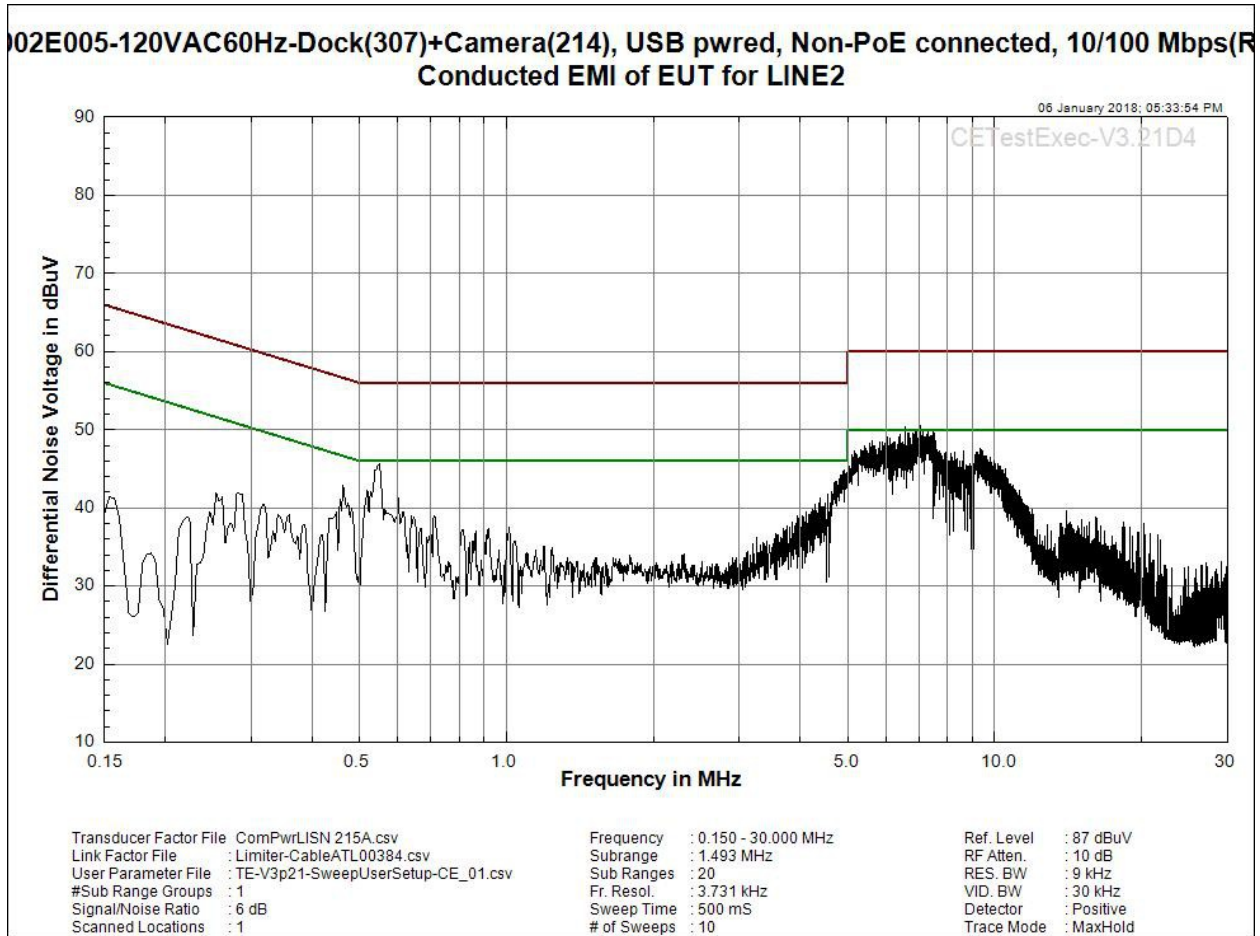
Figure 6.15 - Conducted Emission Scan Line 2 (Line N)
