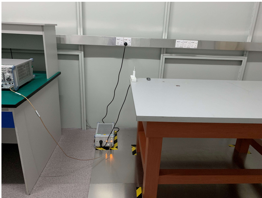
AC Main conducted emission
