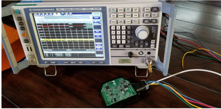
Figure 5: Conducted RF Test Setup Photograph(s).
