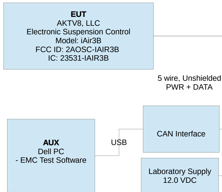
Figure 2: EUT Test Configuration Diagram.
