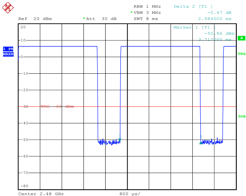
2DH1 time slot (Low, Middle, High Channels)
