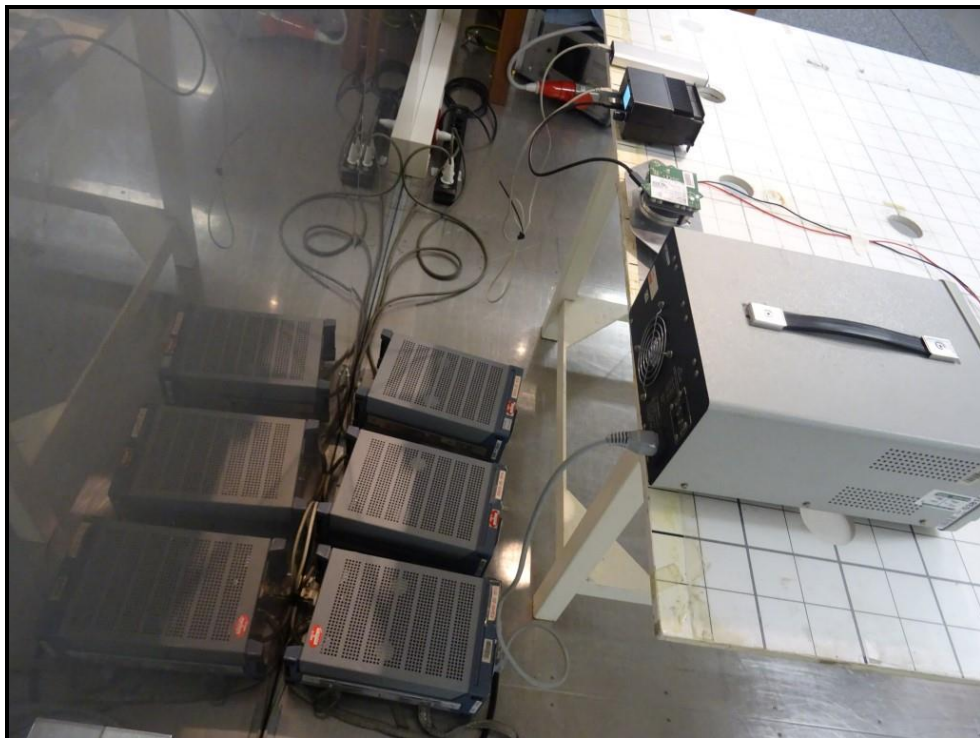
Photo 6 :AC Conducted Emissions WPT TX Module View + WPT RX Module
