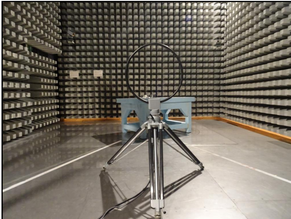
Photo 4: Transmitter H-field & Radiated Spurious Domain Emissions (<30 MHz)
