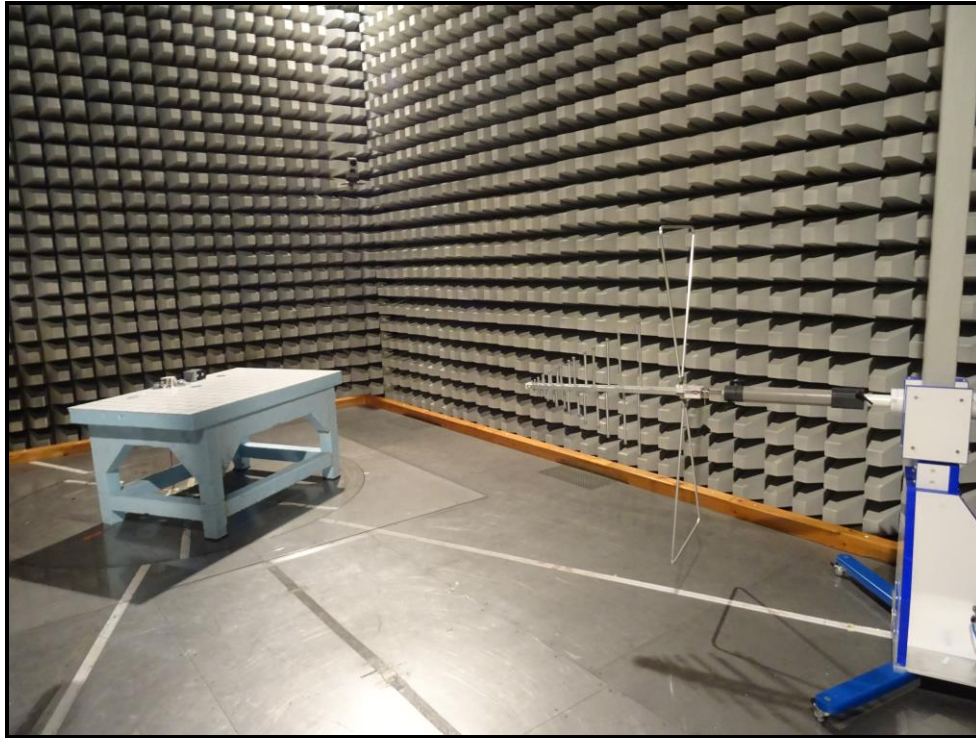
Photo 3 : Radiated Spurious Domain Emissions (>30 MHz)
