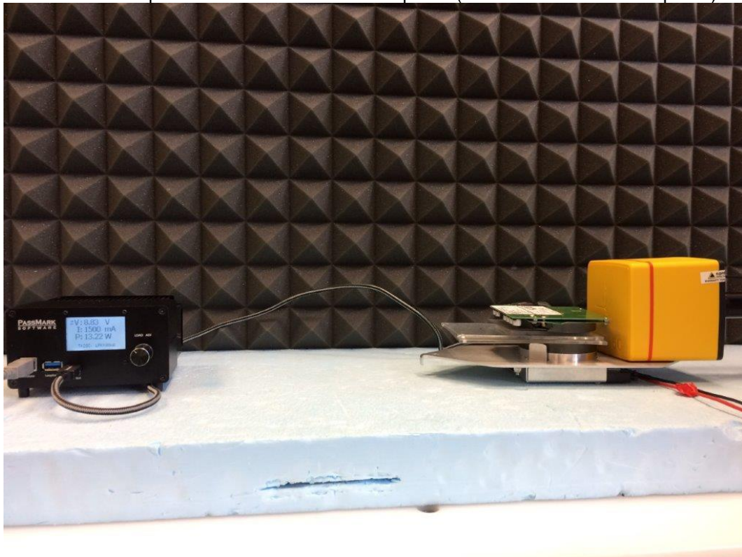
Photo 10: Test position – side 3 with EHP50F probe (15cm to the centre of the probe)
