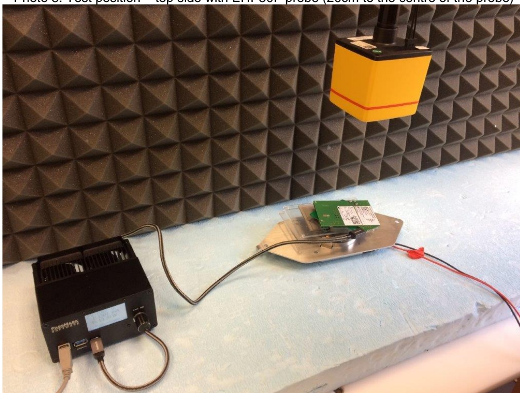
Photo 8: Test position – top side with EHP50F probe (20cm to the centre of the probe)
