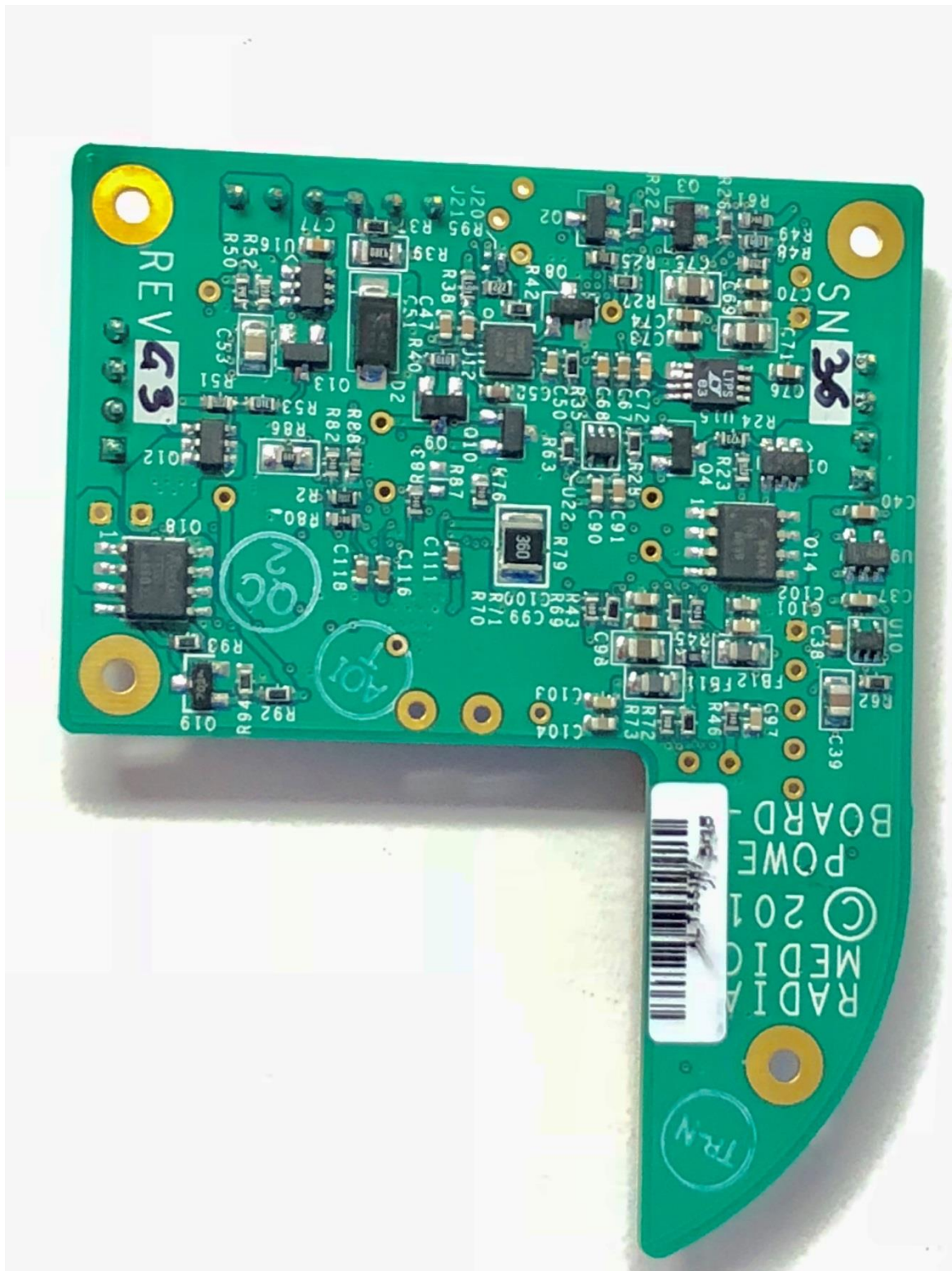
Power Board bottom
