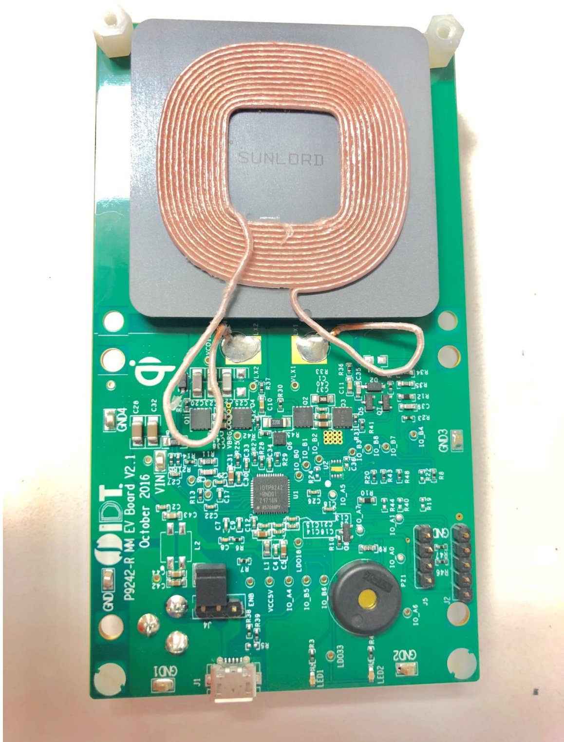
Charger board top
