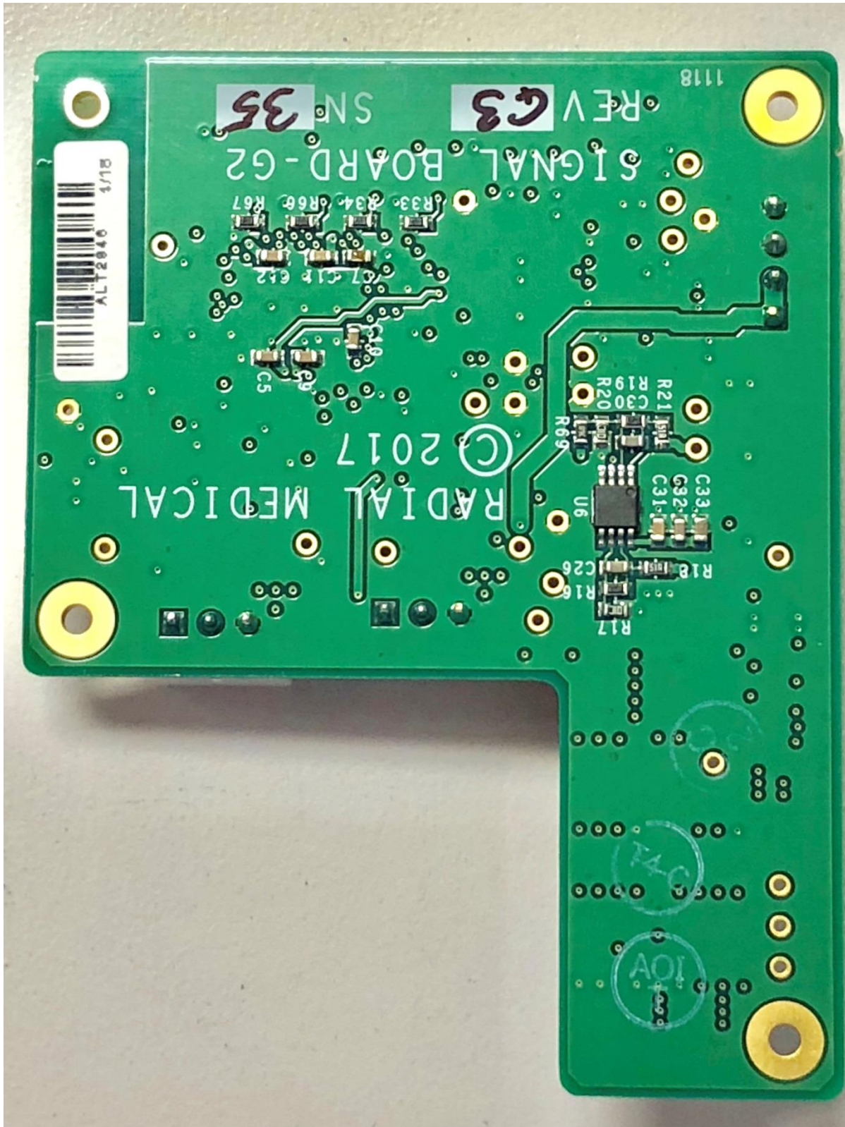
Signal Board Bottom
