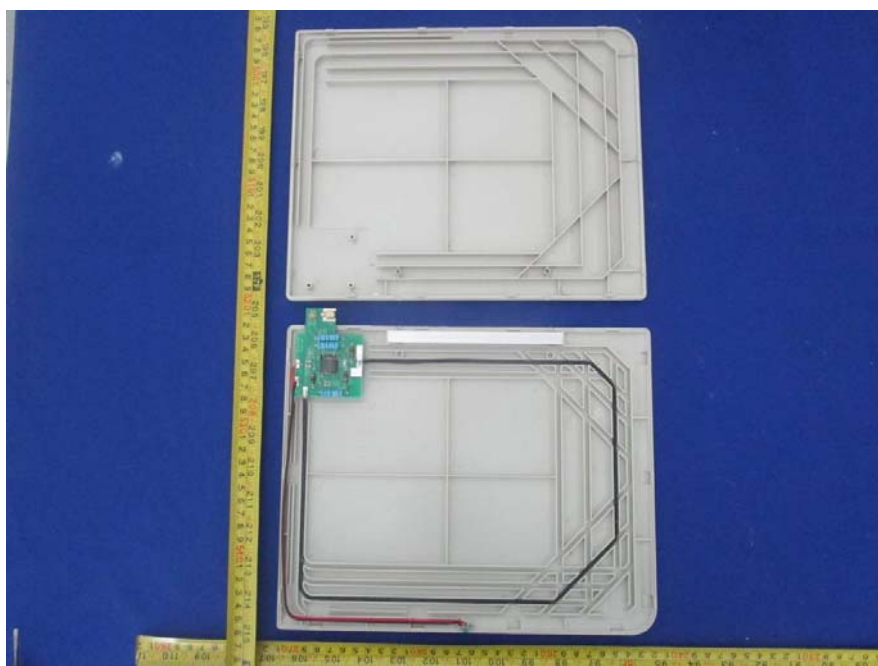
EUT – ANT Uncover1 View
