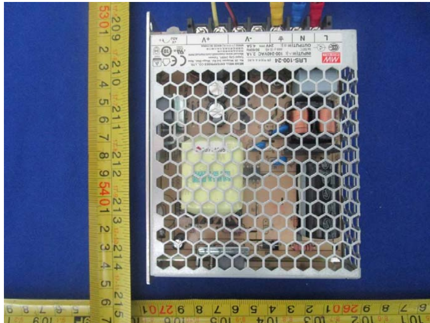
EUT – Power2 Top View
