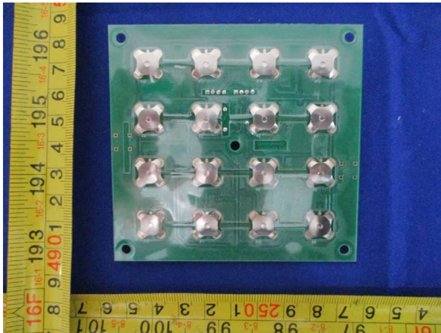
EUT – Keyboard Board Bottom View
