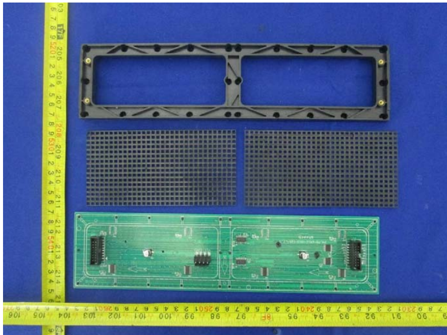
EUT – LED Uncover View
