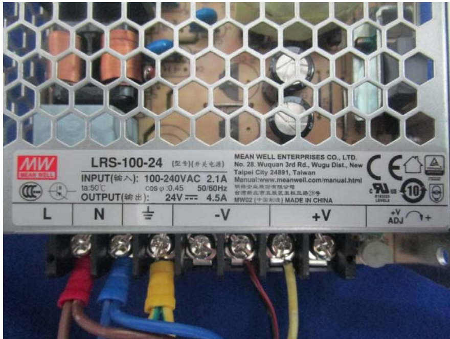
EUT – Power2 Label View
