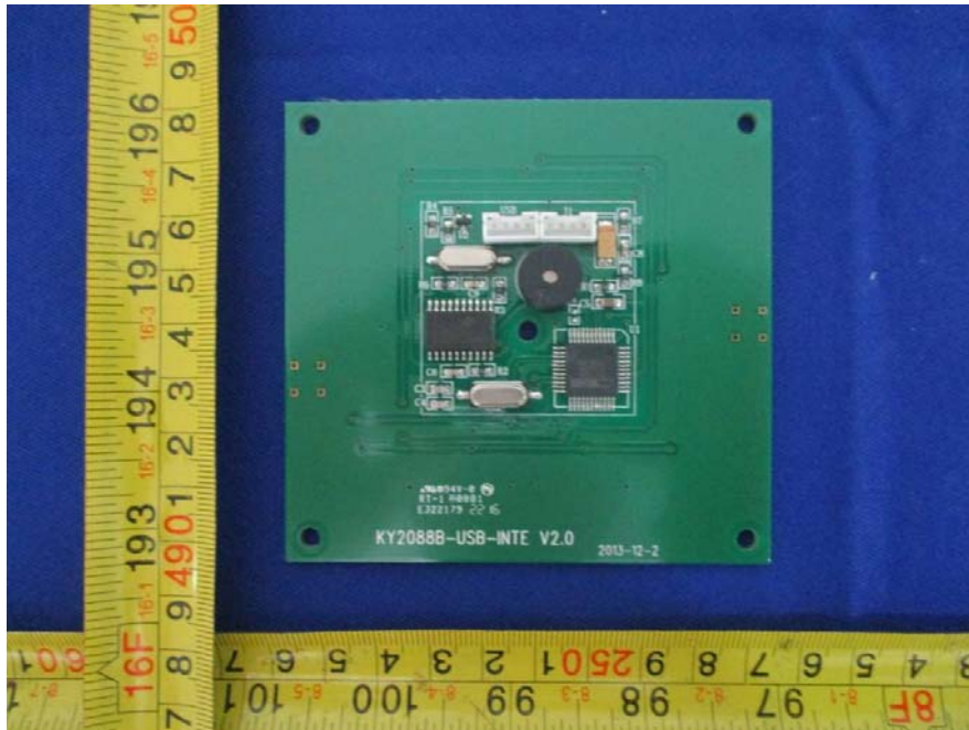
EUT – Keyboard Board Top View
