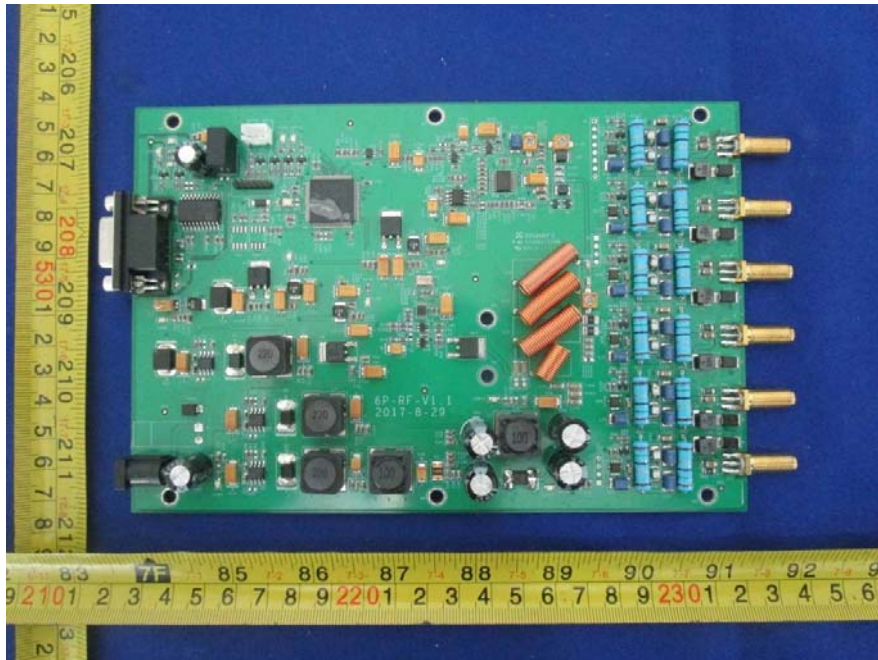
EUT – Signal Box PCB Top View
