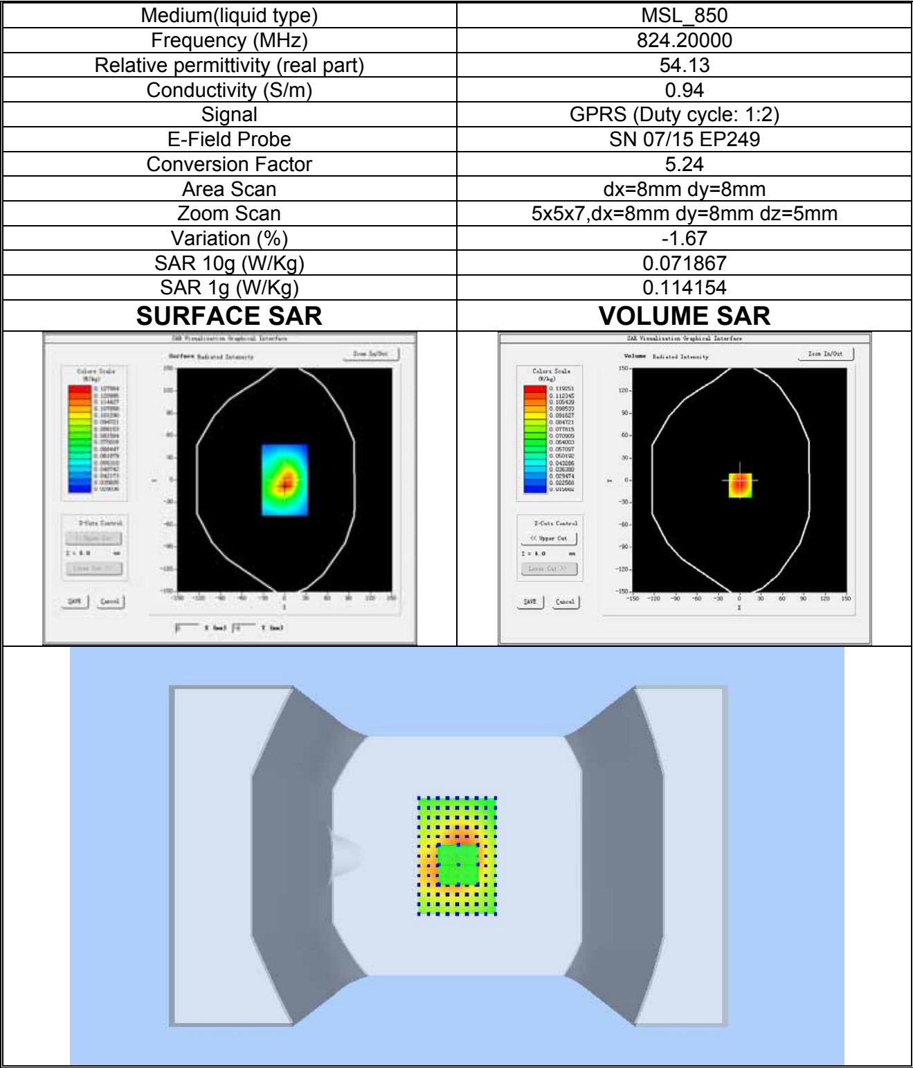
Plot 8: GPRS850MHz, Low channel(Body-worn, Bottom edge) Product Description: Mobile Phone Test Date: 2018-01-28
