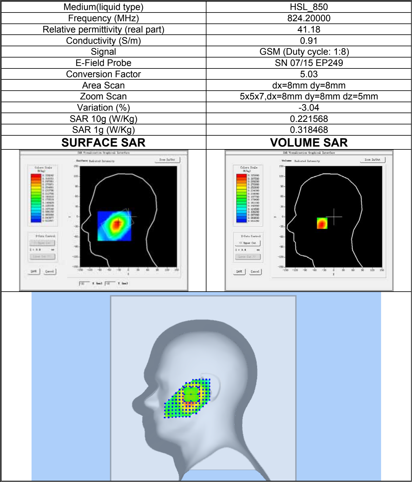
Plot 2: GSM850MHz, Low channel (Right Head , Tilt) Product Description: Mobile Phone Test Date:2018-01-28
