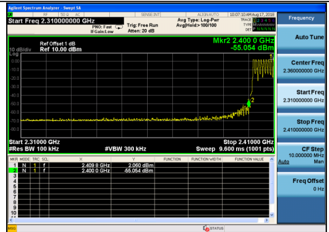
Hopping-on mode
