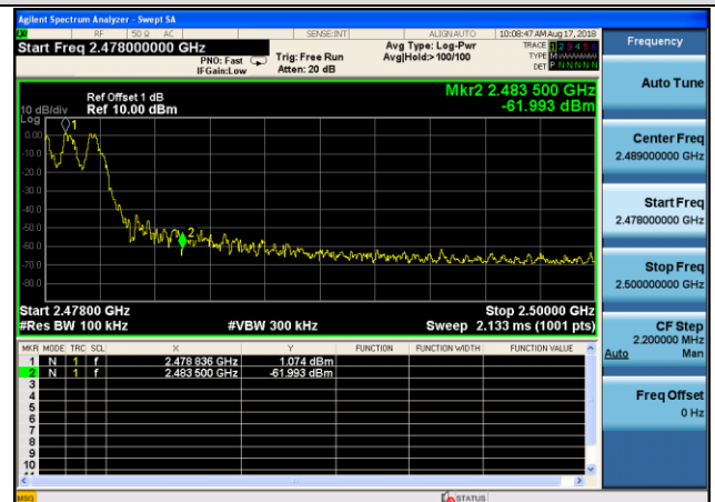
Hopping-on mode
