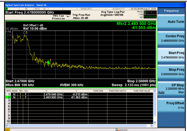
Hopping-on mode
