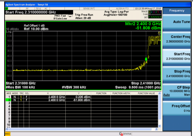
Hopping-on mode
