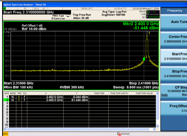
Hopping-off mode
