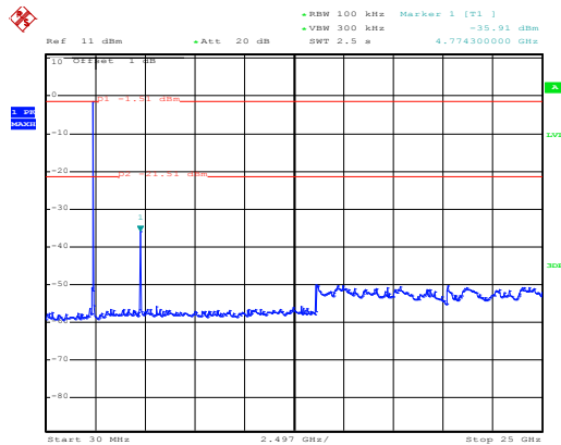
GFSK Lowest channel
