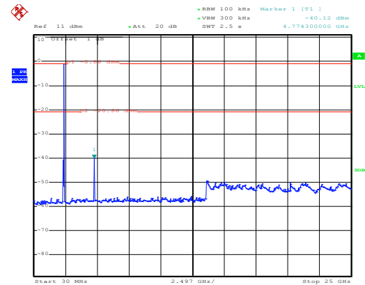
\pi/4 -DQPSK Lowest channel
