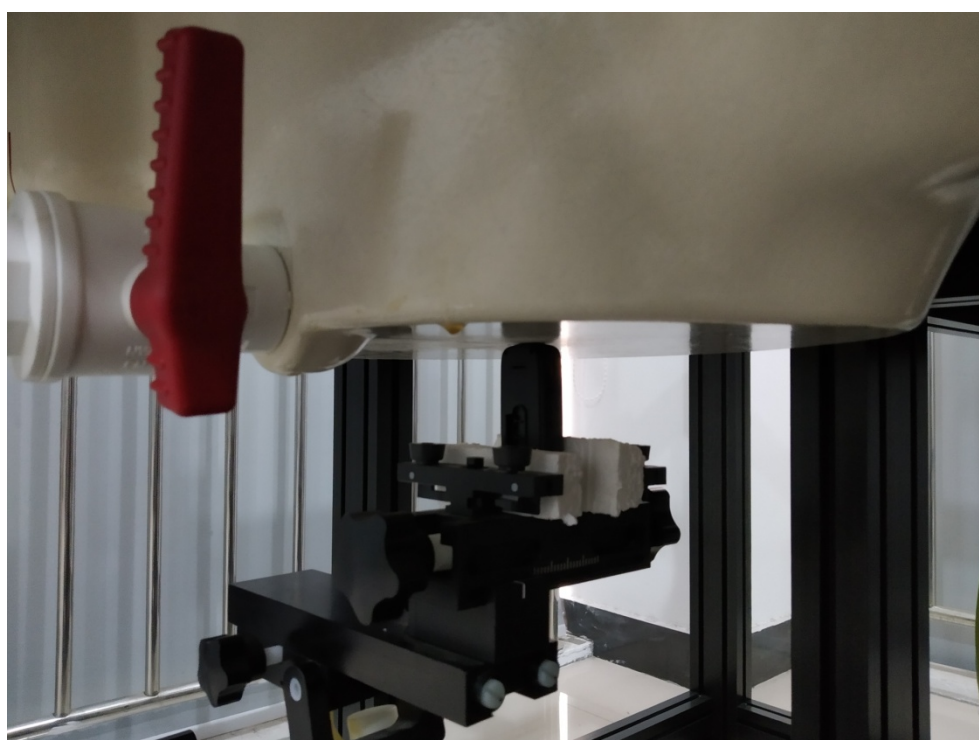
Bottom Side Touch to Flat Phantom (0 mm) Setup Photo
