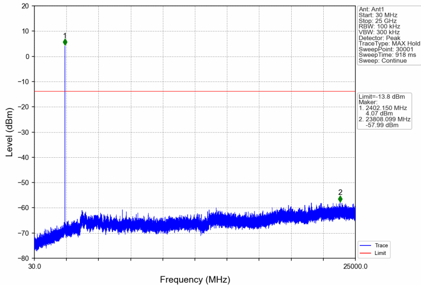
8DPSK_3DH5_LCH_2402MHz_Ant1_NTNV
