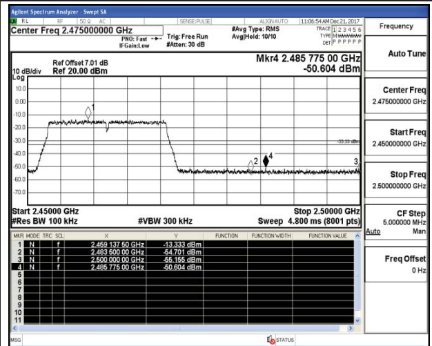
Channel 11 / 2462 MHz
