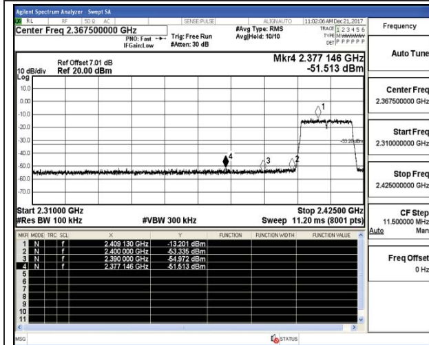
Channel 1 / 2412 MHz
