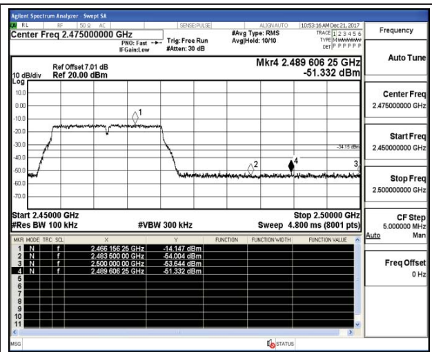
Channel 11 / 2462 MHz
