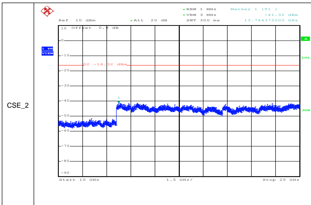
RF Conducted Spurious Emissions_11G_2412_Ant1
