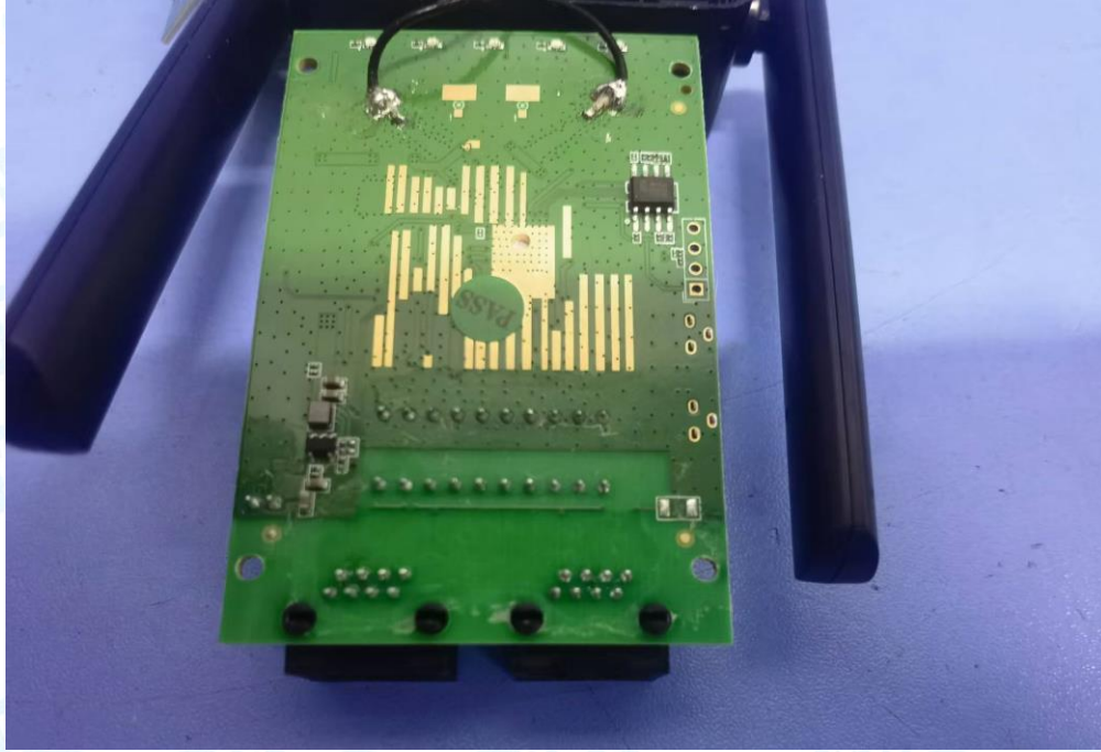
Photo 13 Internal of EUT
