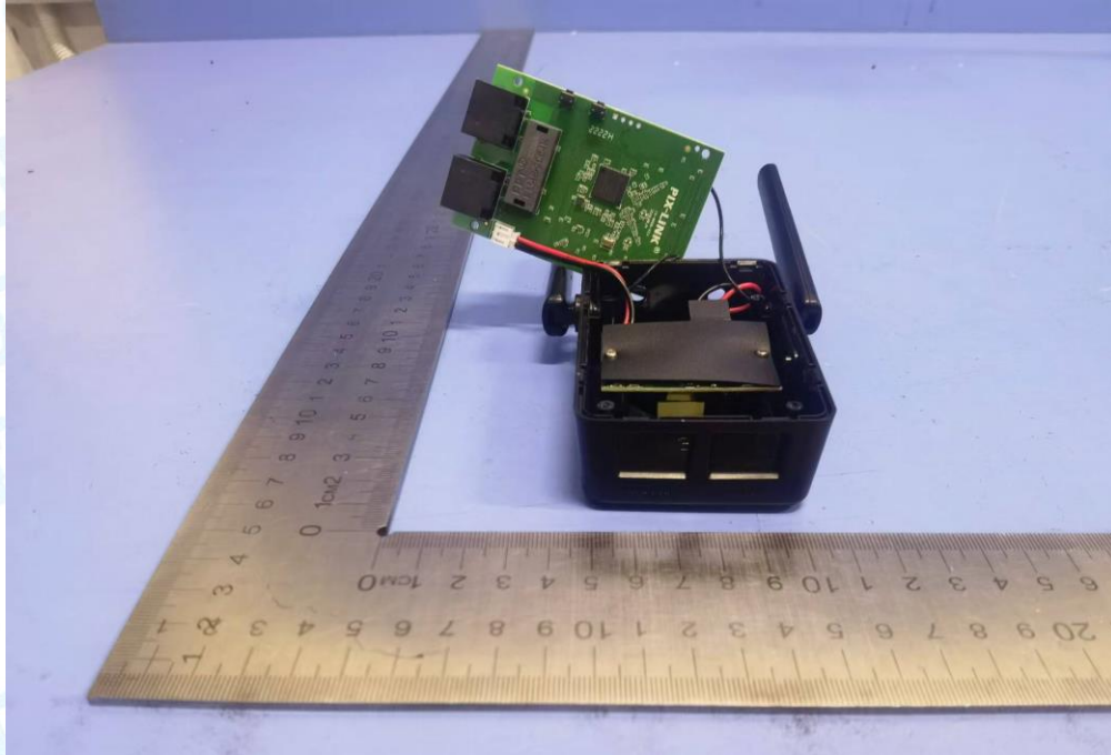
Photo 9 Internal of EUT
