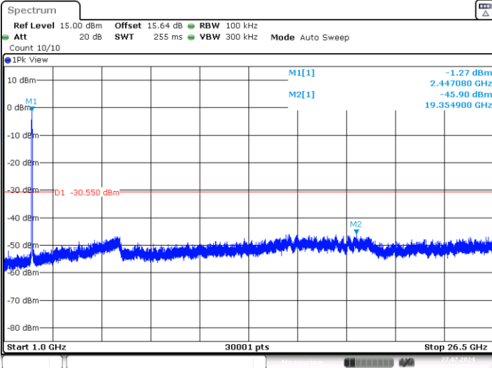
11N40-CDD-Ant1-2452-0~Reference-PASS
