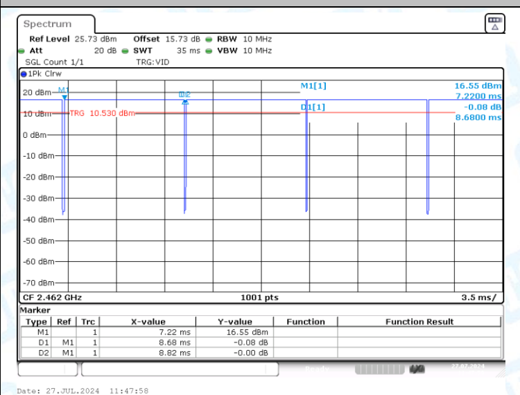
NTNV-11B-CDD-Ant2-2462
