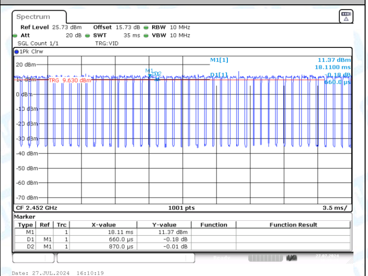
NTNV-11N40-CDD-Ant2-2452
