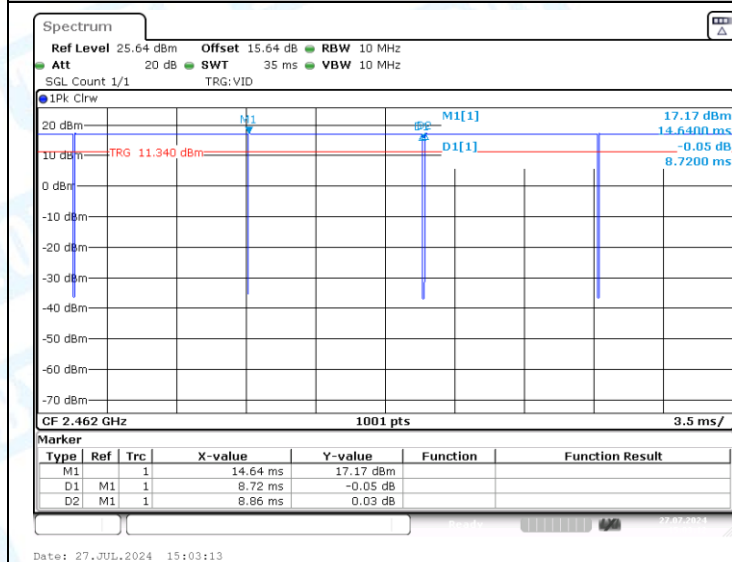
NTNV-11B-Ant1-2462
