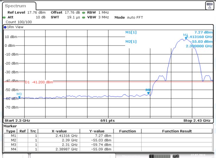
11B-CDD-Ant1-2412-PASS
