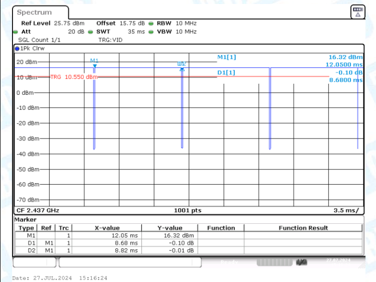
NTNV-11B-Ant2-2437
