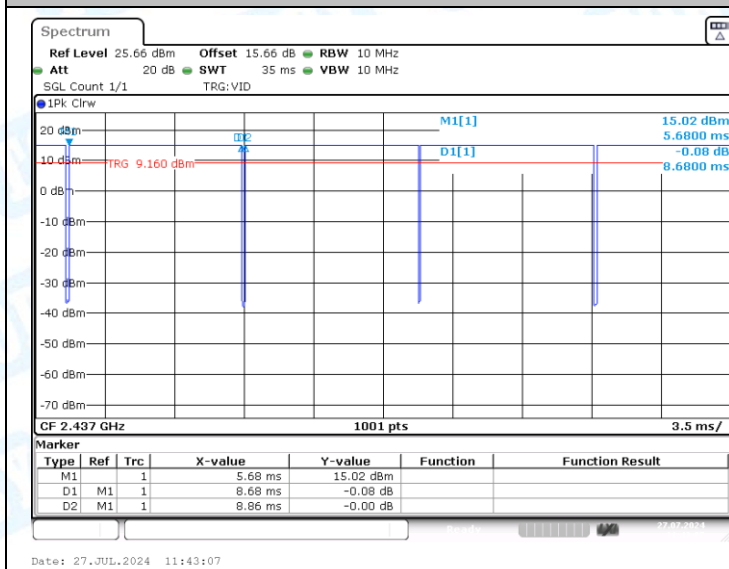
NTNV-11B-CDD-Ant1-2437
