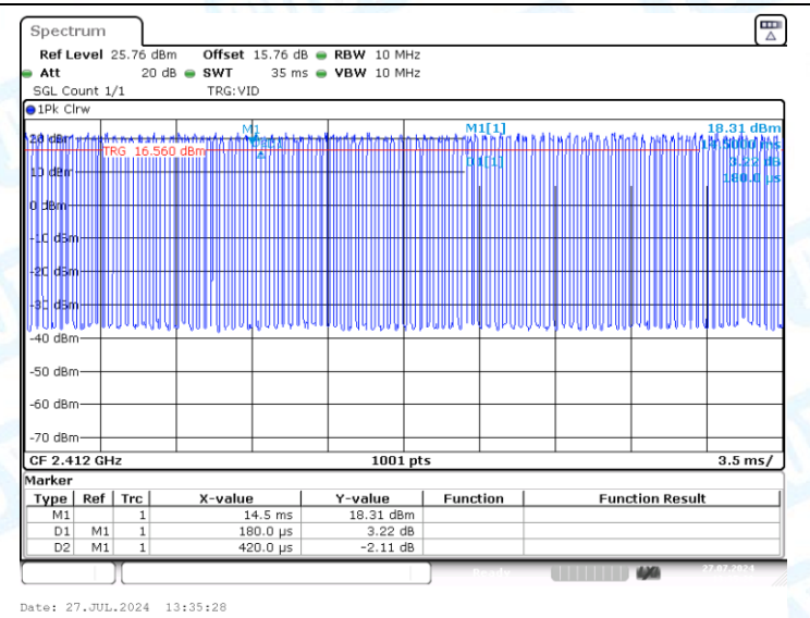
NTNV-11G-CDD-Ant2-2412
