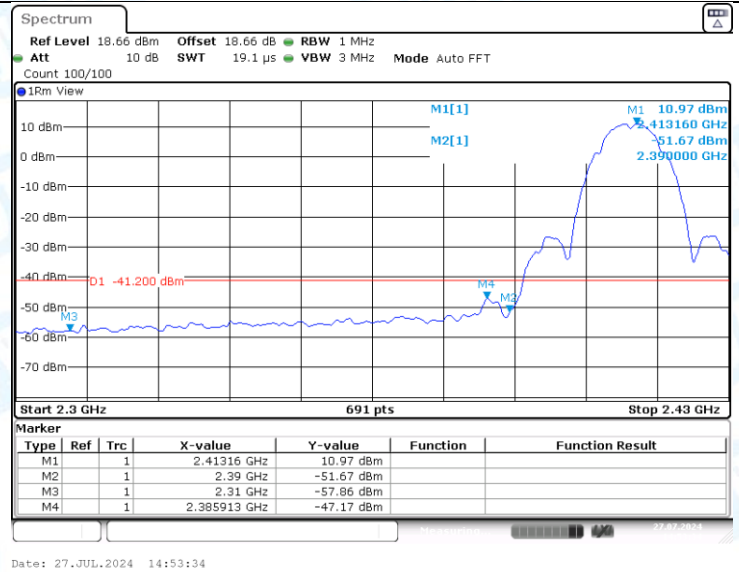
11B-Ant1-2412-PASS
