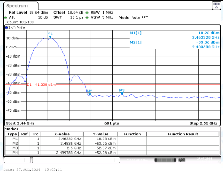
11B-Ant1-2462-PASS
