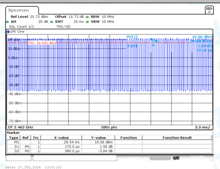
NTNV-11G-CDD-Ant2-2462
