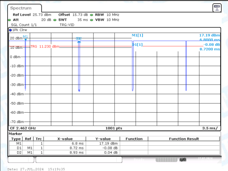
NTNV-11B-Ant2-2462
