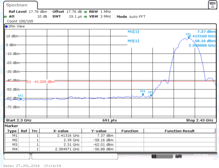
11B-Ant2-2412-PASS
