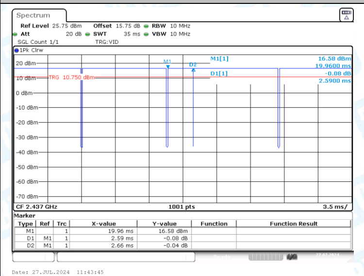
NTNV-11B-CDD-Ant2-2437
