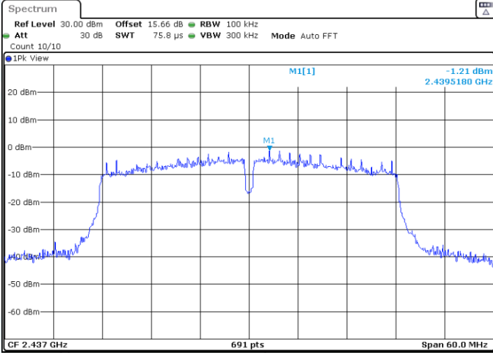
11N40-CDD-Ant1-2437-0~Reference-PASS
