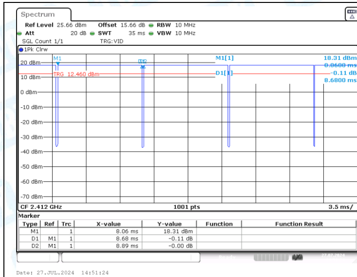
NTNV-11B-Ant1-2412
