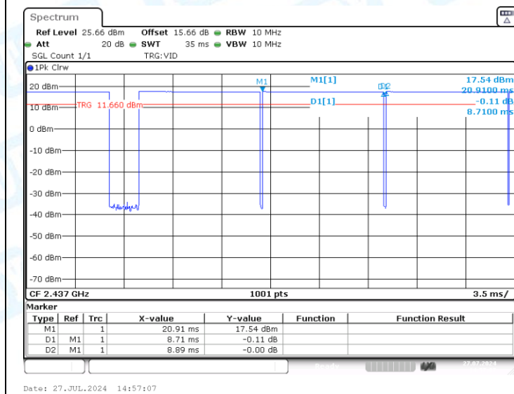
NTNV-11B-Ant1-2437
