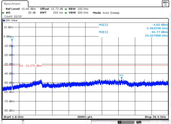
11N40-CDD-Ant2-2452-0~Reference-PASS
