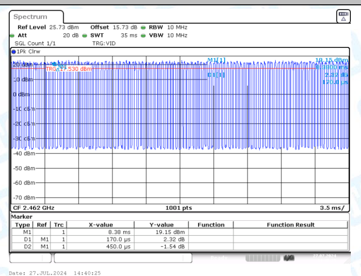
NTNV-11G-Ant2-2462
