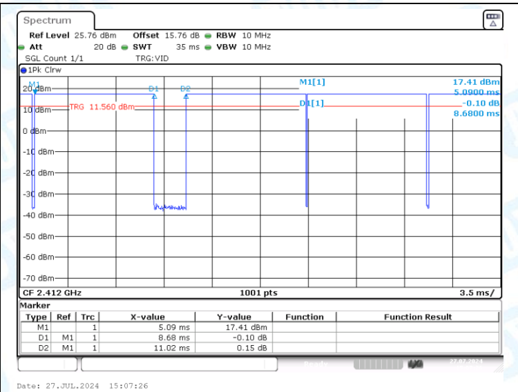
NTNV-11B-Ant2-2412
