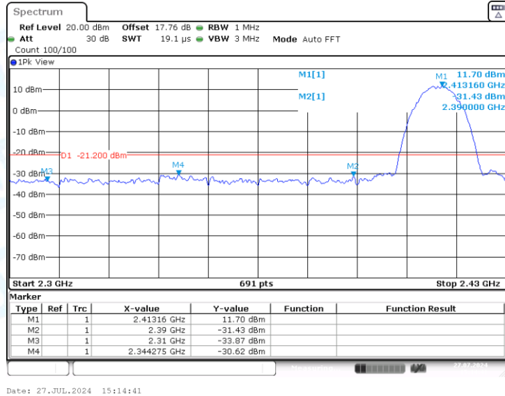
11B-Ant2-2412-PASS
