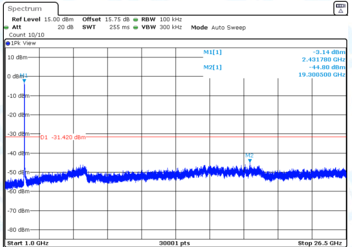
11N40-CDD-Ant2-2437-0~Reference-PASS
