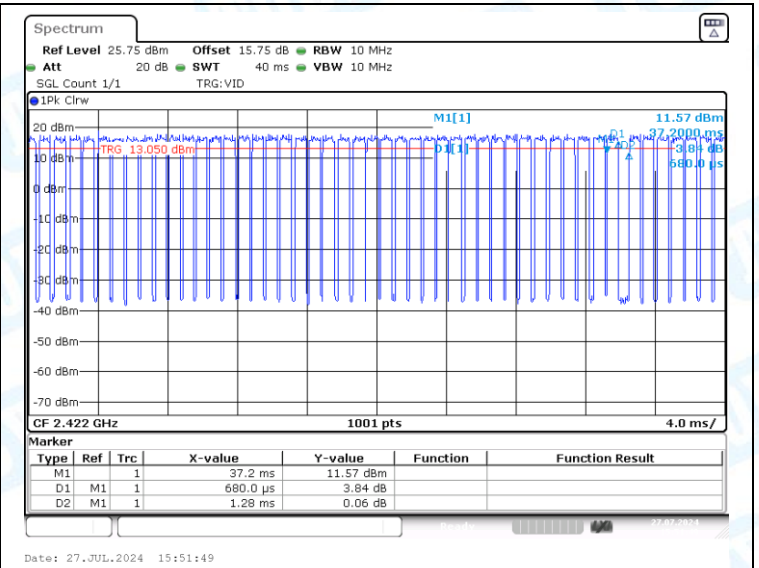
NTNV-11N40-CDD-Ant2-2422
