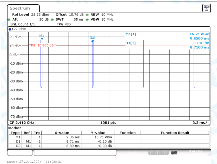
NTNV-11B-CDD-Ant2-2412
