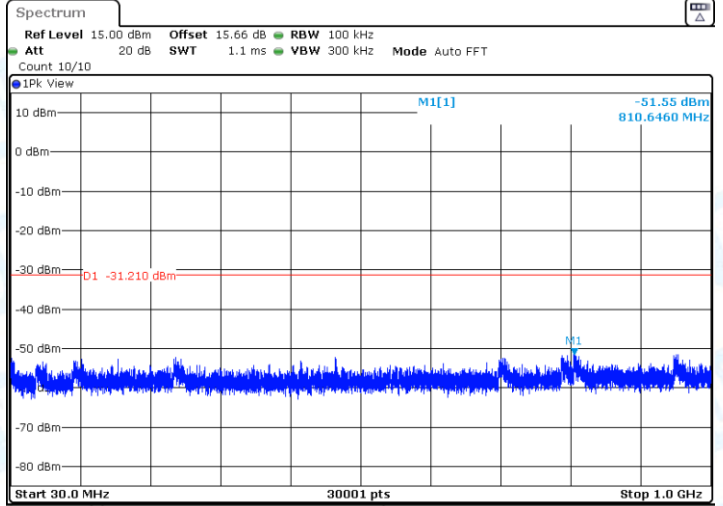
11N40-CDD-Ant1-2437-30~1000-PASS
