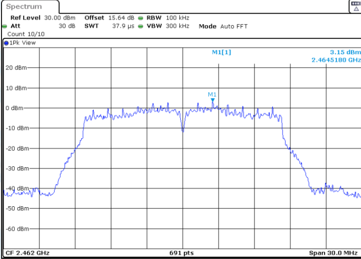
11G-CDD-Ant1-2462-0~Reference-PASS
