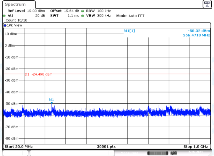
11B-Ant1-2462-30~1000-PASS
