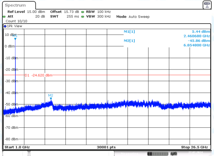
11B-Ant2-2462-0~Reference-PASS
