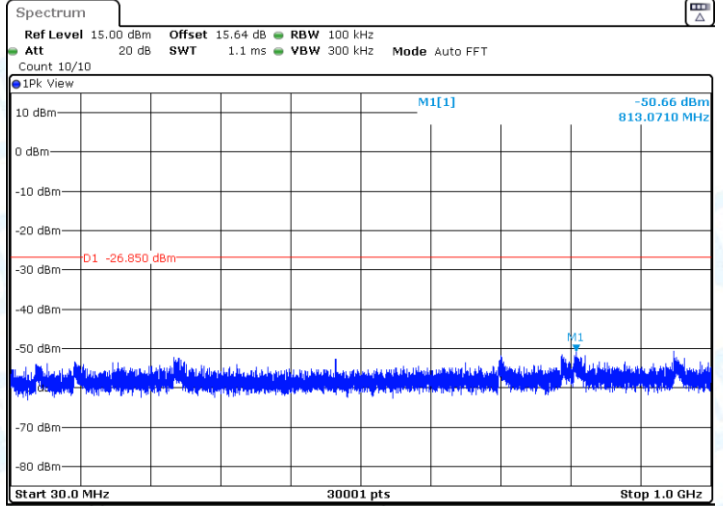
11G-CDD-Ant1-2462-30~1000-PASS
