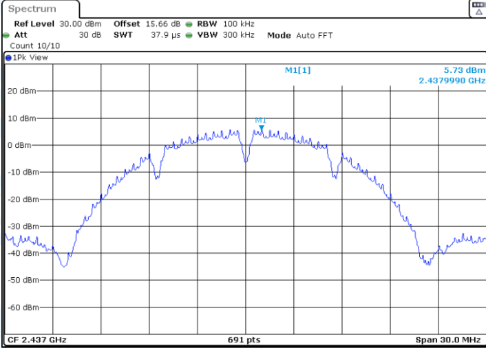
11B-Ant1-2437-0~Reference-PASS
