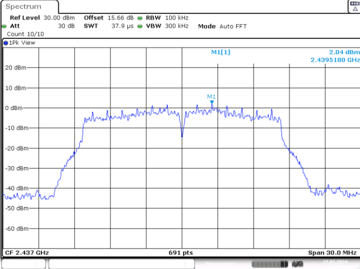
11G-CDD-Ant1-2437-0~Reference-PASS
