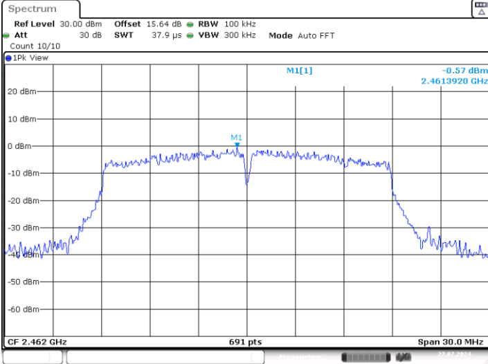
11N20-CDD-Ant1-2462-0~Reference-PASS
