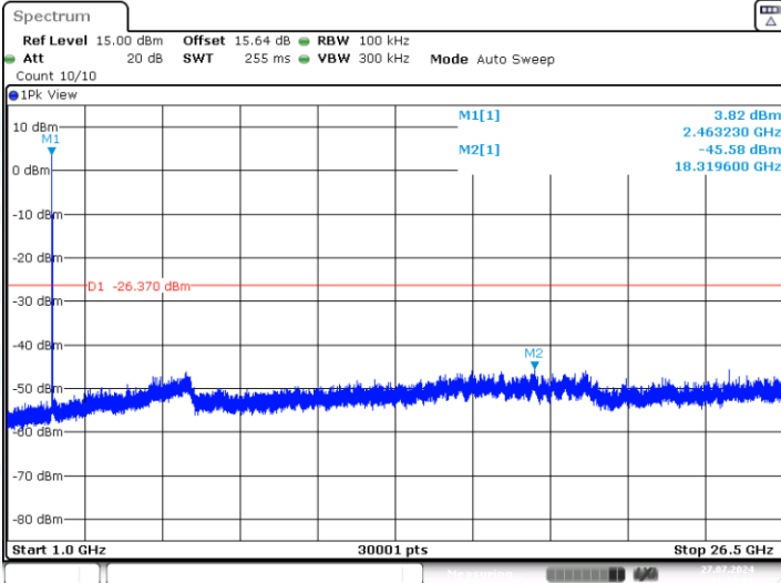
11B-CDD-Ant1-2462-0~Reference-PASS
