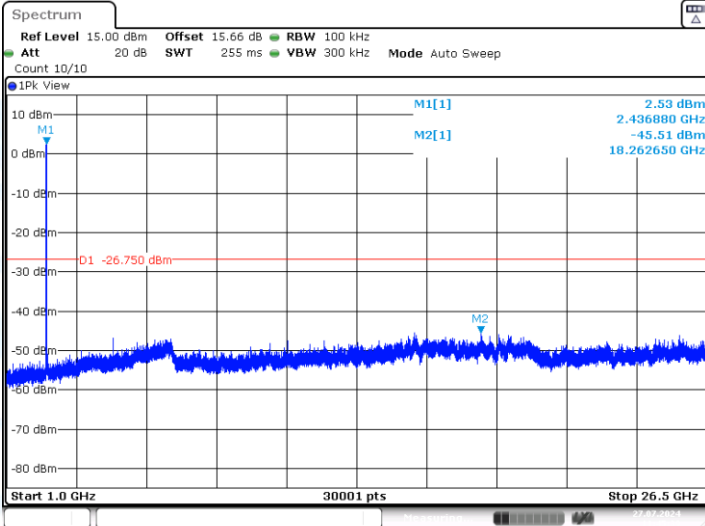
11B-CDD-Ant1-2437-0~Reference-PASS
