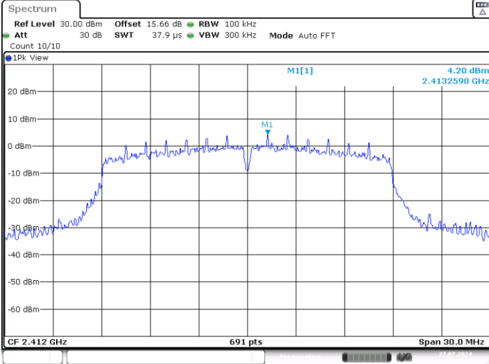
11N20-CDD-Ant1-2412-0~Reference-PASS
