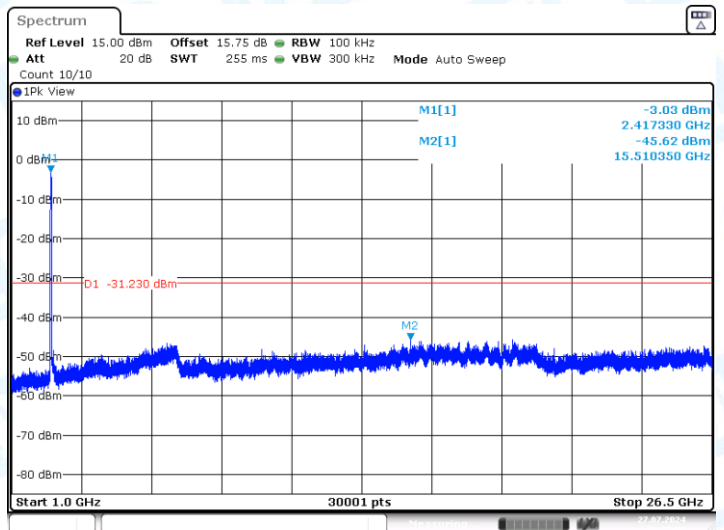
11N40-CDD-Ant2-2422-0~Reference-PASS
