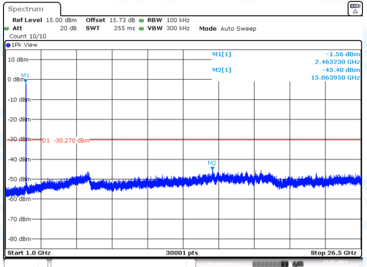
11N20-CDD-Ant2-2462-0~Reference-PASS
