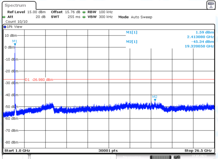
11N20-CDD-Ant2-2412-1000~26500-PASS
