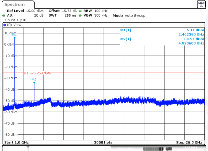
11B-CDD-Ant2-2462-0~Reference-PASS
