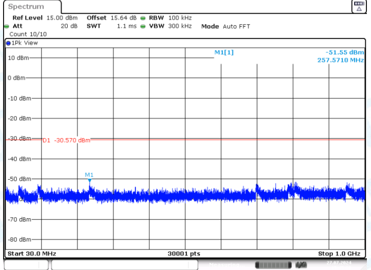
11N20-CDD-Ant1-2462-30~1000-PASS
