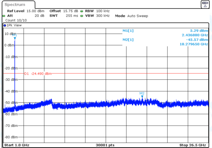
11B-Ant2-2437-0~Reference-PASS
