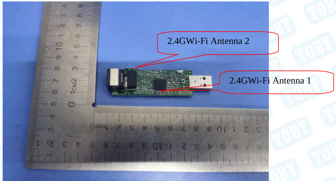
Photo 10 Appearance of PCB
