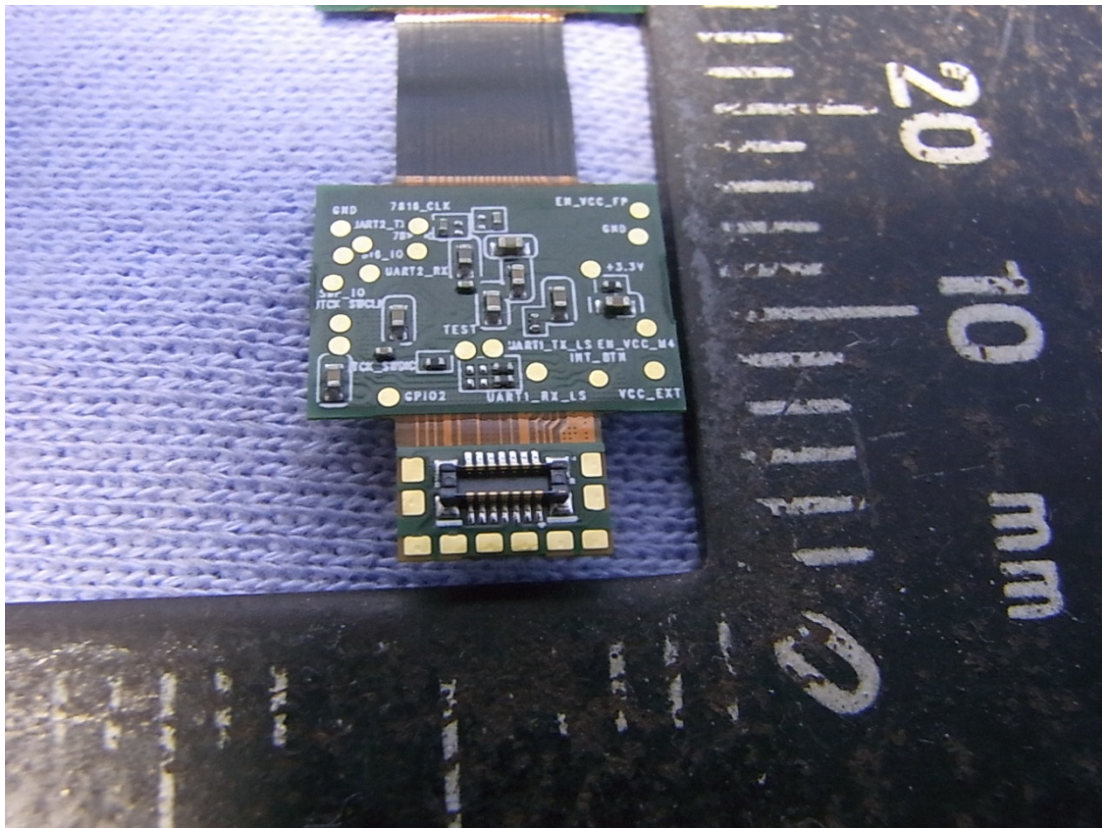
Figure 10 Internal View (Internal Board, Back View)
