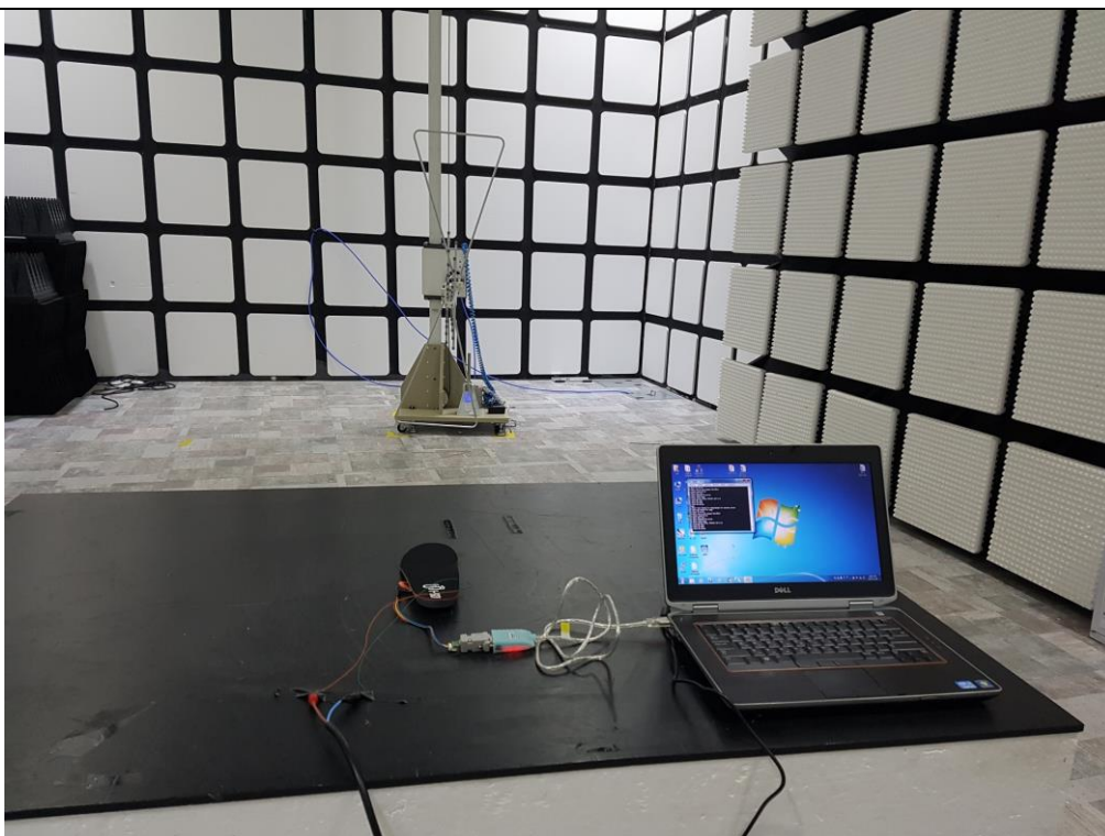
Radiated Test (Below 1G)
