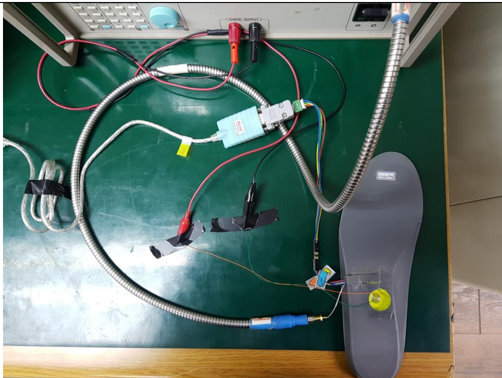
Conducted Test 1
