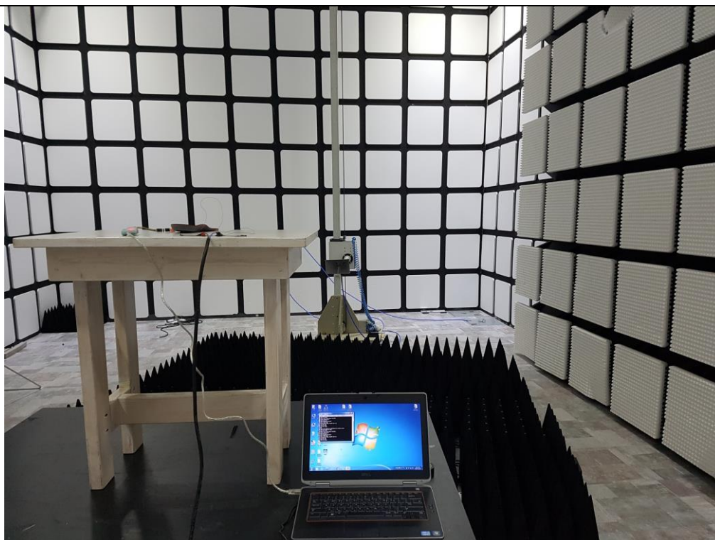
Radiated Test (Above 1G)
