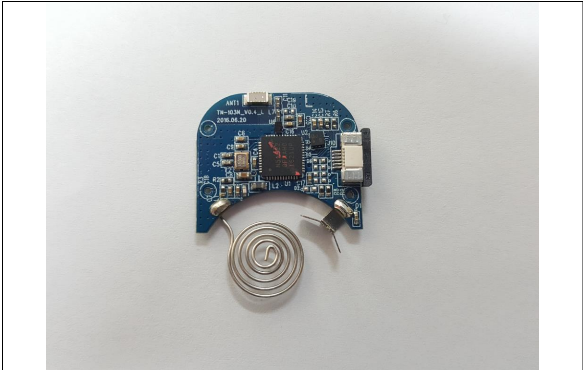
Board (Top)
