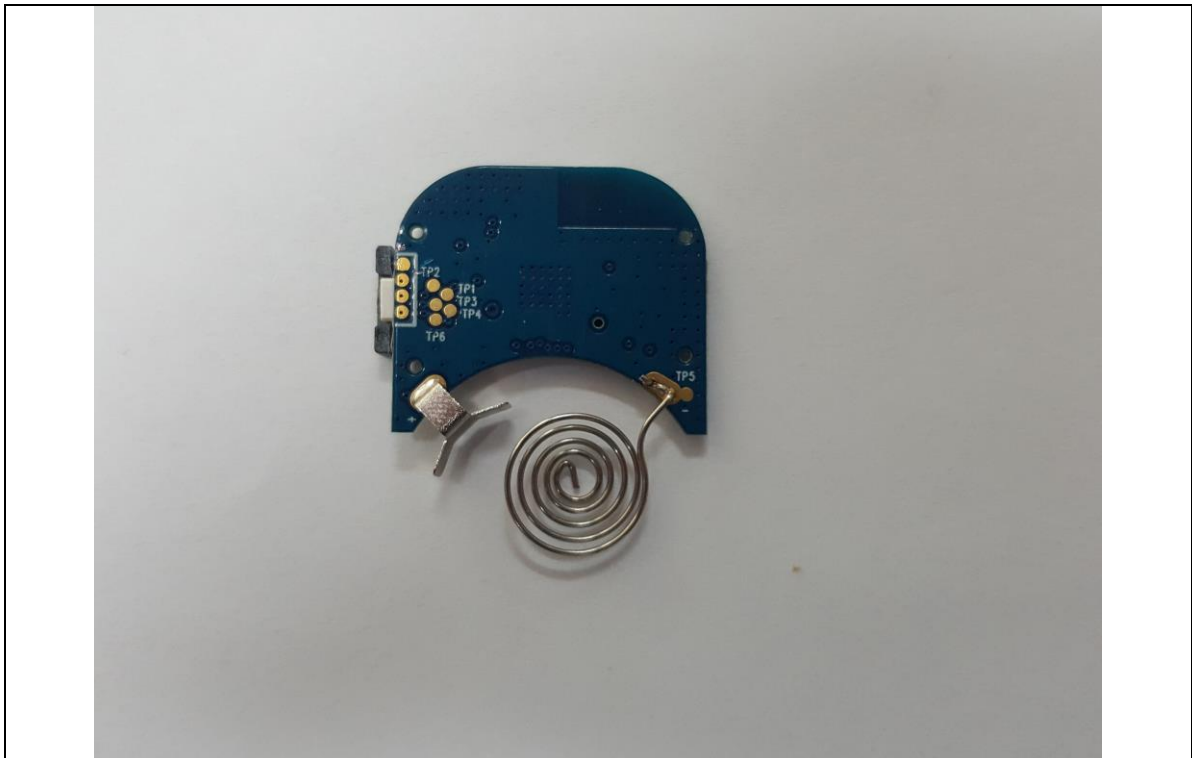
Board (Bottom)
