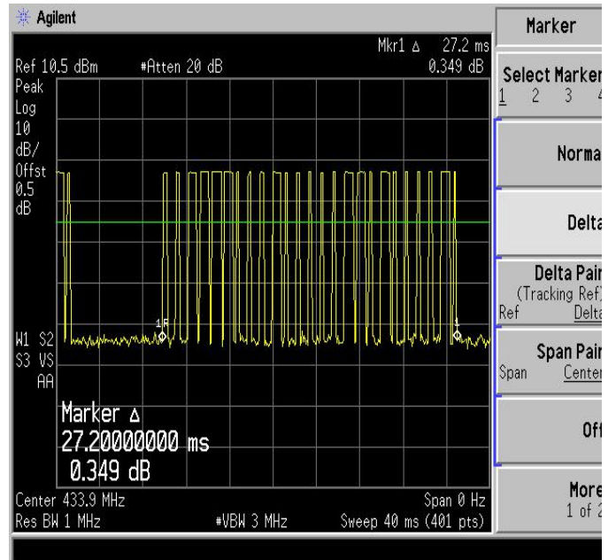
T on time slot-2
