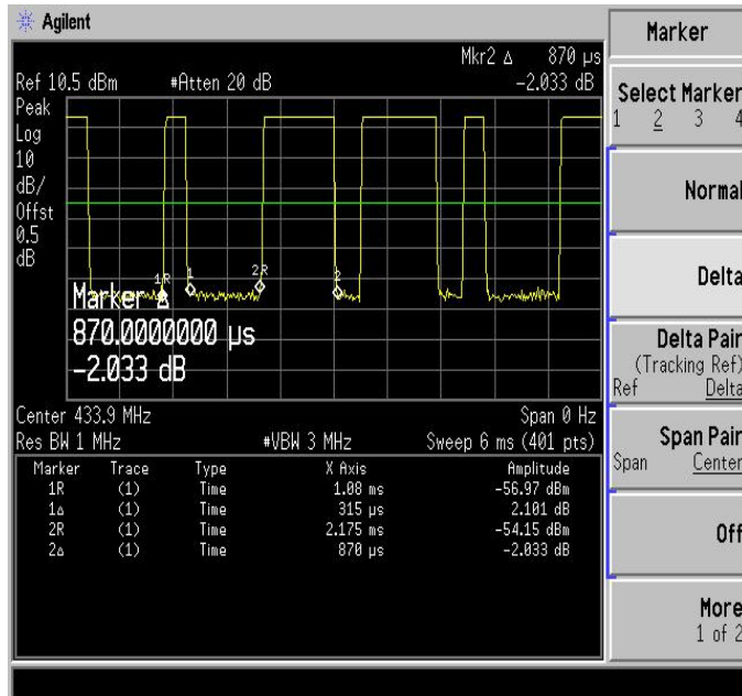
T on time slot-1
